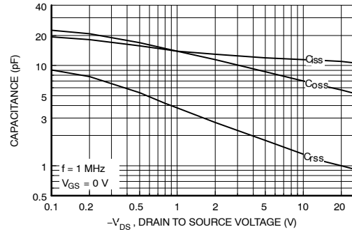
Figure 18. Capacitance Characteristics
