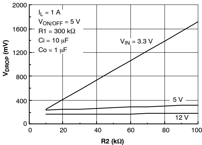
Figure 12. V_{\text{DROP}} Variation with V_{IN} and R_2
