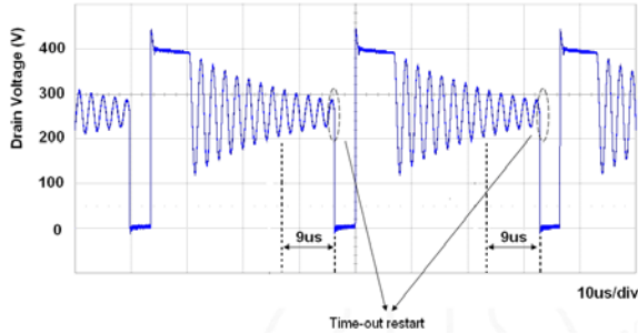
Figure 20. Internal t_{\text{TIME-OUT}} Initiates New Cycle after Failure to Detect Valley Voltage (with 5 µs Delay for FAN6300H version)
