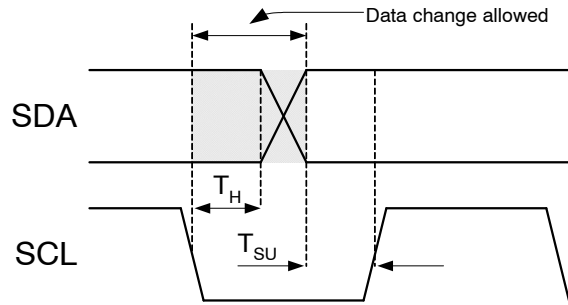
Figure 49. Data Transfer Timing
