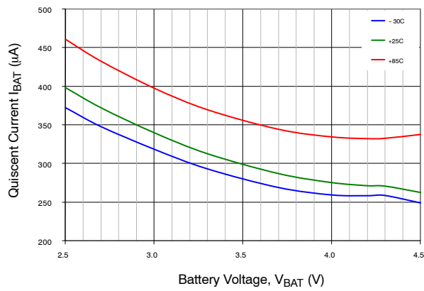
Figure 36. Quiescent Current
