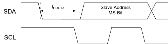
Figure 34. START Bit
