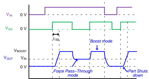
Figure 17. Pass-Through Profile
