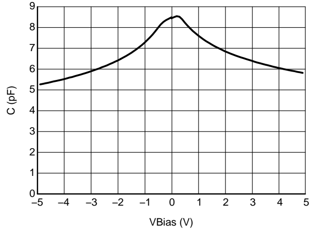
Figure 4. CV Characteristics
