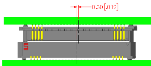
INITIAL X AXIS LINEAR MISALIGNMENT
