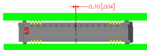
FINAL X AXIS LINEAR MISALIGNMENT
