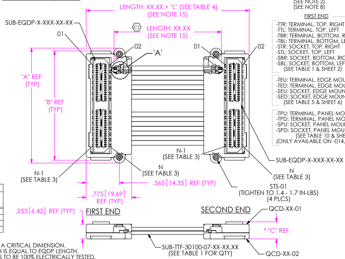
FIG 1 VERTICAL (EQDP-028-XX.XX-STR-STR-1 SHOWN)
