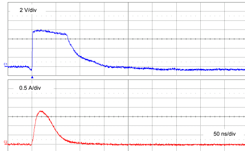
Figure 10. ISO7637-3 pulse 3b response ( V_S = 100 V)
