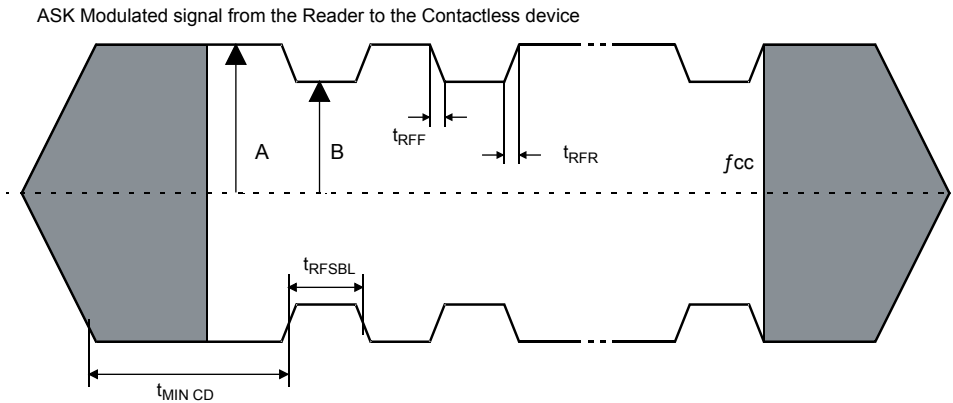
Figure 46. ST25TB02K synchronous timing, transmit and receive
