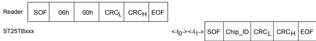
Figure 47. Initiate frame exchange between reader and ST25TB02K
