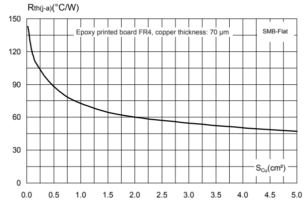
Figure 6. Thermal resistance junction to ambient versus copper surface under each lead
