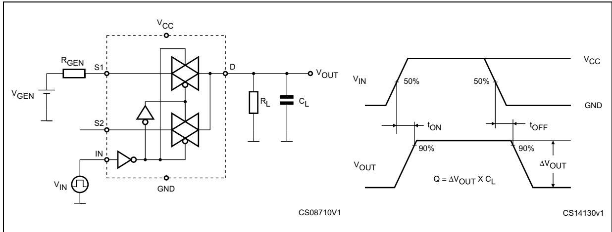
Figure 11. Switching time and charge injection (V GEN = 0 V, R GEN = 0 Ω, R L = 1 MΩ, C L = 100 pF)
