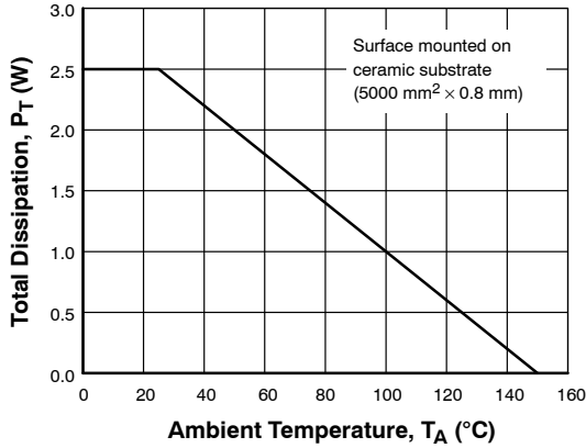
Figure 10. Total Dissipation vs. Temperature
