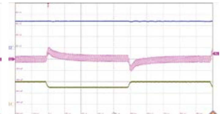
Ch1: Input voltage (10 V/div.) Ch4: Output current (500m A/div) Ch2: Output voltage (100 mV/div.) Time scale: (100 us/div.)
