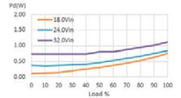
Power dissipation vs load
