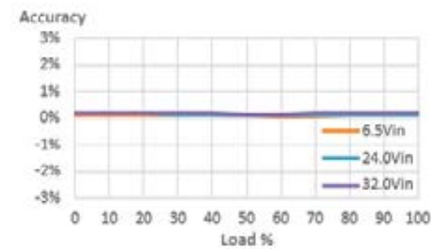
Accuracy vs load
