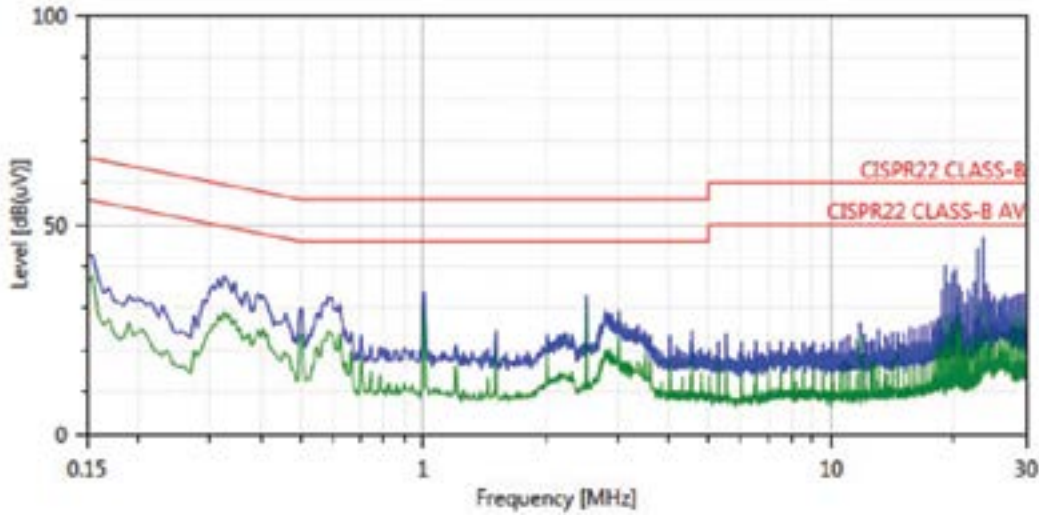
With Class B filter Blue line: Peak Band: 0.15 - 30 MHz Green line: Average
