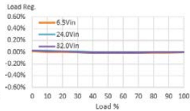
Load regulation vs load
