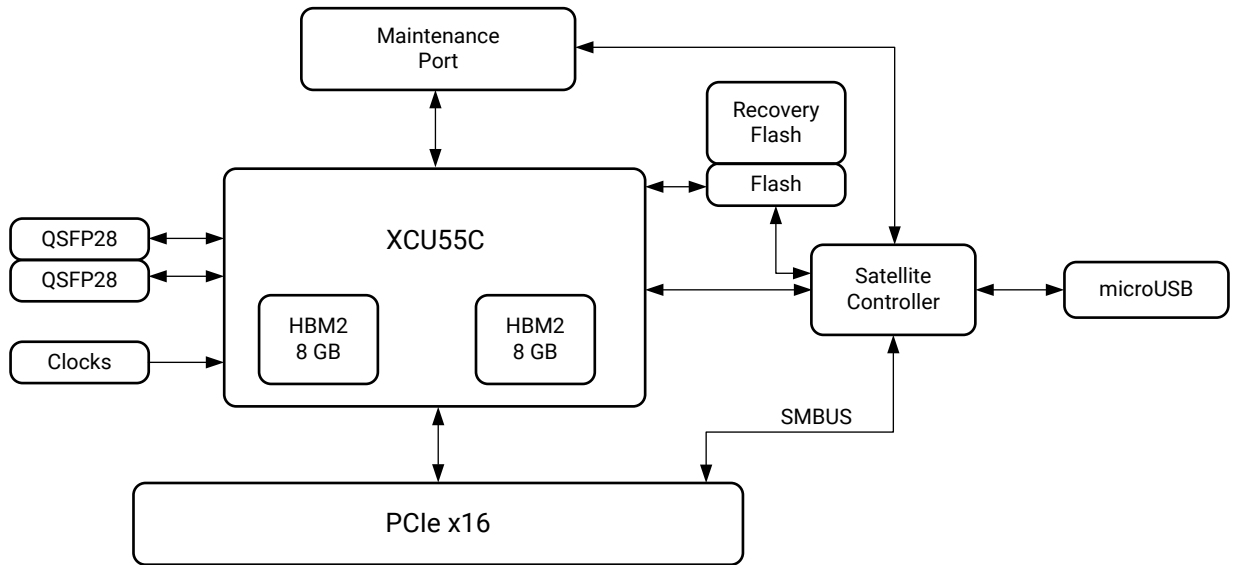
Figure 2: XCU55C Block Diagram
