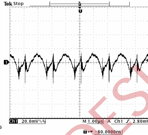
48 Vdc input, 5.0 Vdc output
