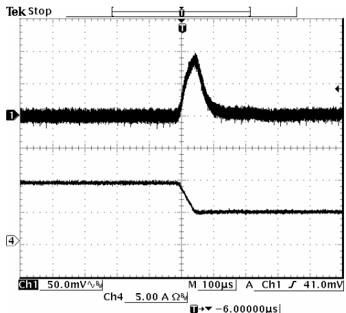
Vout=1.2 V 50% to 25% Load Transients
