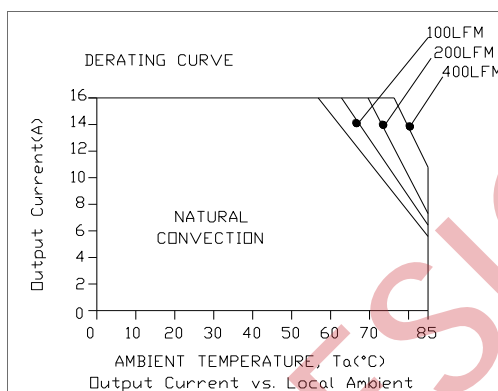
xRSB-40UV5x, Vin=75V
