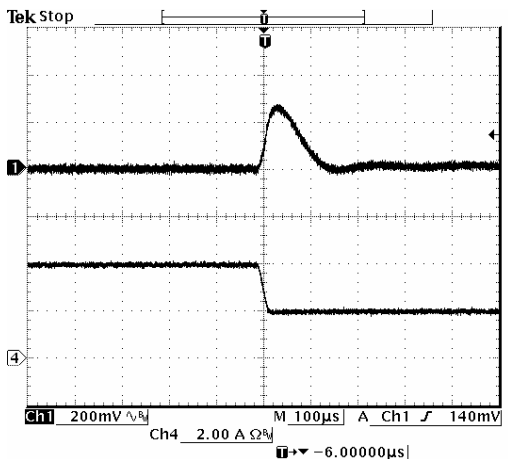
Vout=5.0 V 50% to 25% Load Transients
