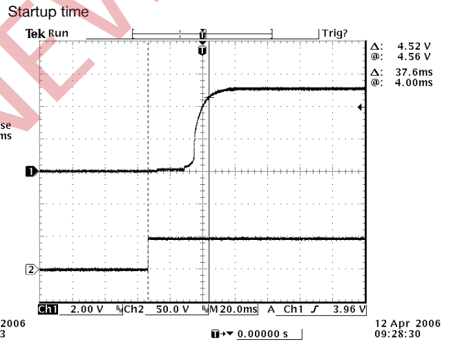
Vout=5V 100% Load at Vin=48V
