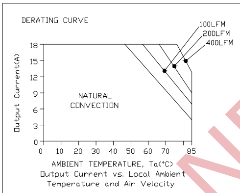
xRSB-40UV2x, Vin=48V
