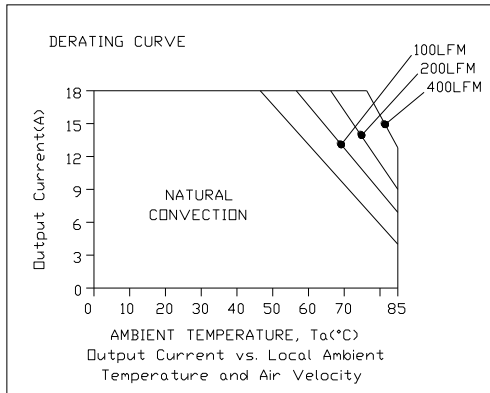
xRSB-40UV2x, Vin=18V
