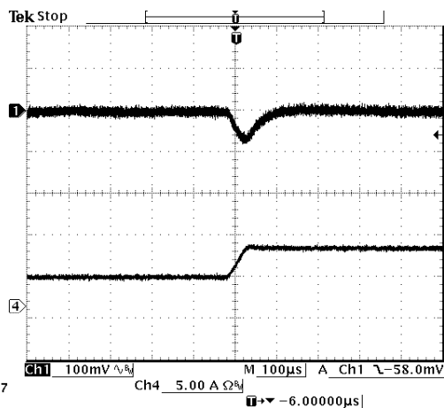
Vout=1.8 V 25% to 50% Load Transients
