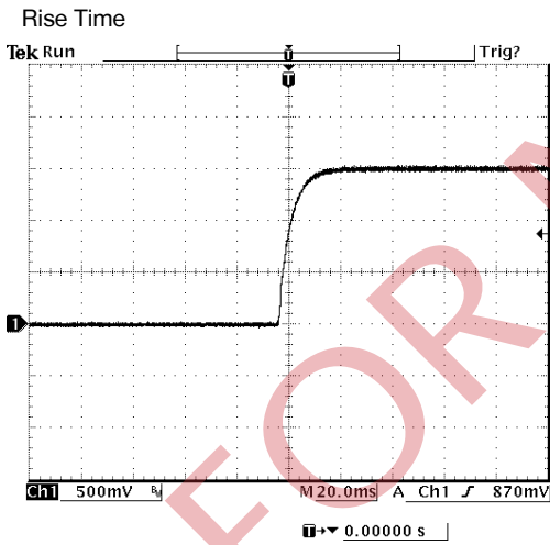
Vout=1.5V 100% Load at Vin=48V
