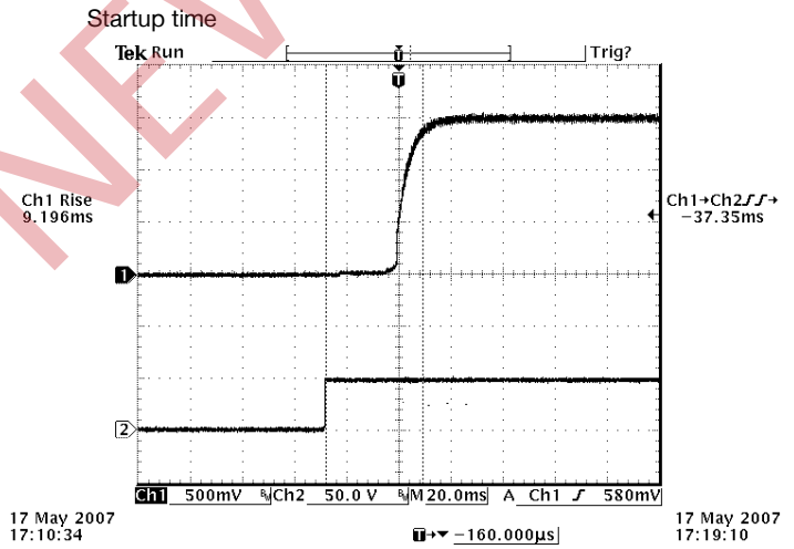
Vout=1.5V 100% Load at Vin=48V
