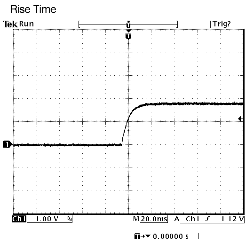
Vout=1.8V 100% Load at Vin=48V
