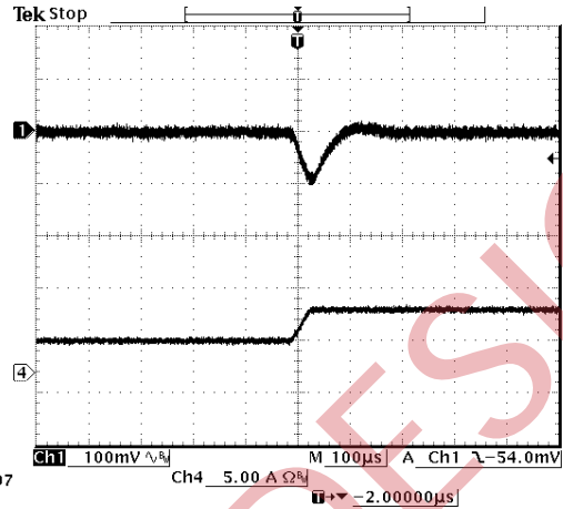
Vout=2.5 V 25% to 50% Load Transients
