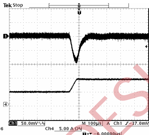
Vout=1.2 V 25% to 50% Load Transients
