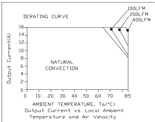
xRSB-40UV5x, Vin=48V
