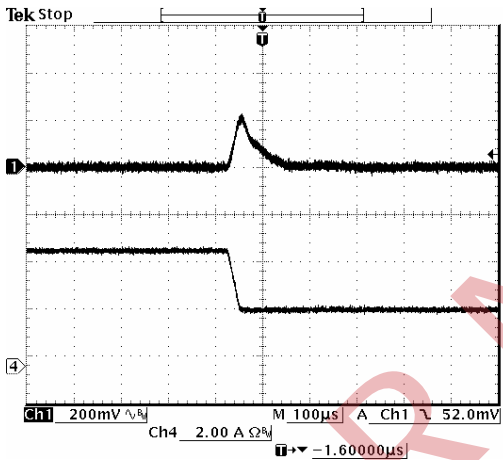
Vout=3.3 V 50% to 25% Load Transients
