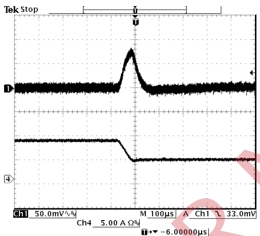
Vout=1.5 V 50% to 25% Load Transients
