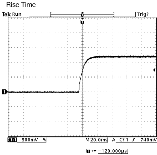
Vout=1.2V 100% Load at Vin=48V
