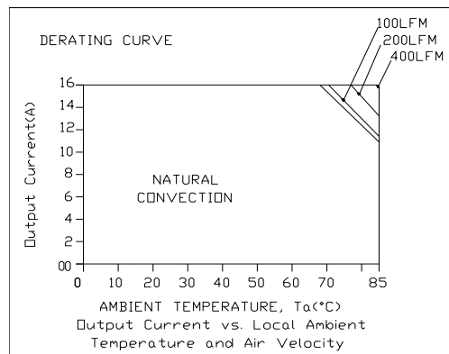
xRSB-40UV5x, Vin=24V
