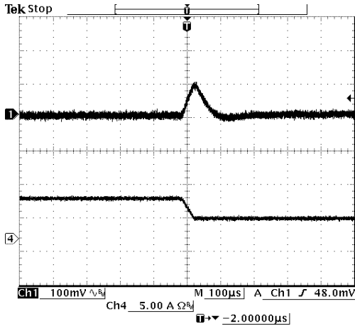
Vout=2.5 V 50% to 25% Load Transients
