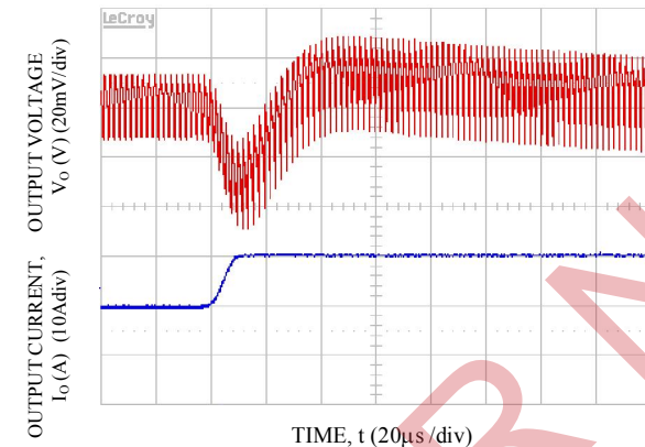
Transient Response to Dynamic Load Change from 50% to 100% at 12Vin, C_{out}= 2x47\mu F +3x330\mu F , C_{Tune}=5600pF & R_{Tune}=220\text{ ohms} . V_o=1.8V
