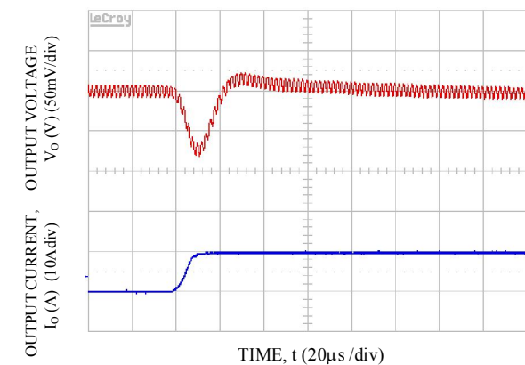
Transient Response to Dynamic Load Change from 50% to 100% at 12Vin, C_{out}= 8x47\mu F , C_{Tune}=1500pF & R_{Tune}=220\text{ ohms} . V_o=5.0V
