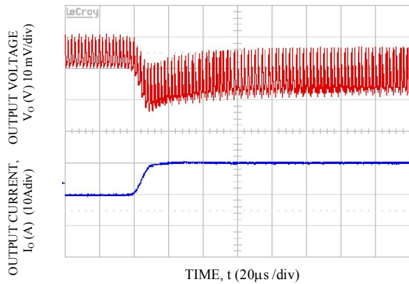
Transient Response to Dynamic Load Change from 50% to 100% at 12Vin, C_{out}= 1x47\mu F +11x330\mu F , C_{Tune}=47nF , R_{Tune}=178\text{ ohms} . V_o=0.6V
