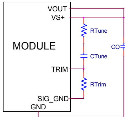
Circuit diagram showing connection of R_{TUNE} and C_{TUNE} to tune the control loop of the module.
