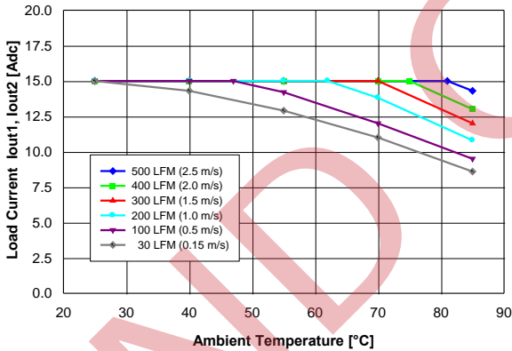
Figure 9. Available balanced load current ( I_{out1} = I_{out2} ) vs. ambient air temperature and airflow rates for converter with D height pins mounted vertically with V_{in} = 48 V, air flowing from pin 3 to pin 1 and maximum FET temperature \leq 120 °C.
