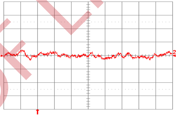
Figure 32. Input reflected ripple current, i_s (10 mA/div), measured through 10\text{ H} at the source at full rated load current on both outputs and V_{in} = 48\text{ V} . Refer to Fig. 30 for test setup. Time scale: 1\text{ }\mu\text{s/div} .
