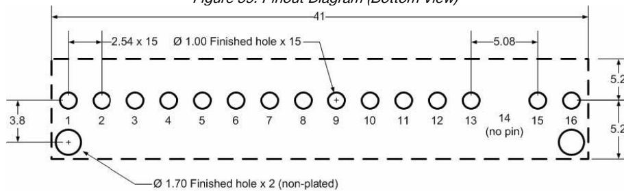
Figure 59. Pinout Diagram (Bottom View)
