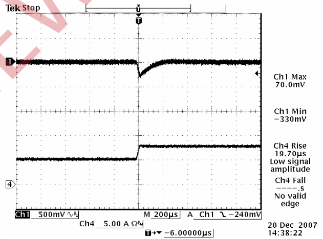
Vo=12 V 50% to 75% Load Transients
