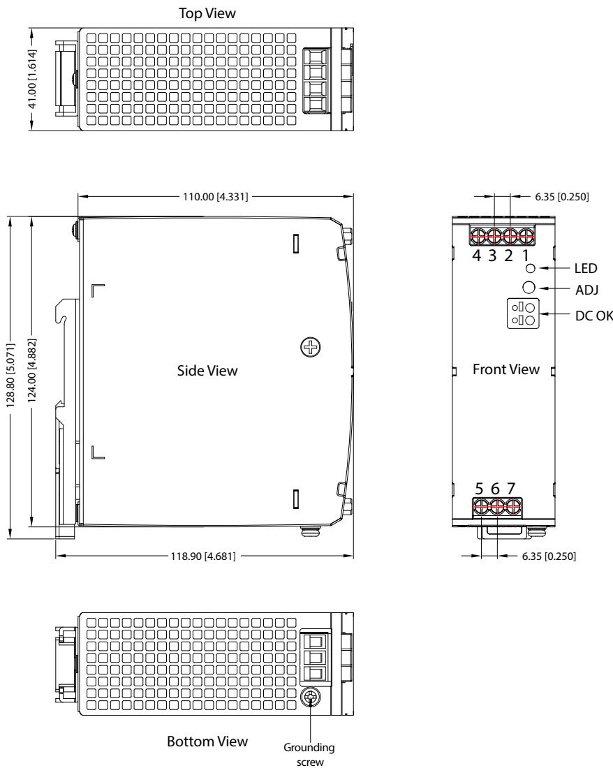
Figure 5. Mechanical Drawing
