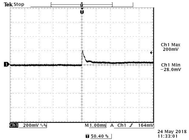
Figure 16. 75%-50% Load Transients at V_{in} = 54 V @ T_a = 25^{\circ}C
