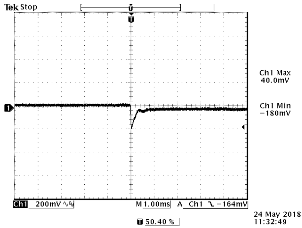
Figure 15. 50%-75% Load Transients at V_{in} = 54 V @ T_a = 25^{\circ}C
