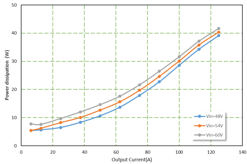
Figure 7. Output Current vs Power Dissipation
