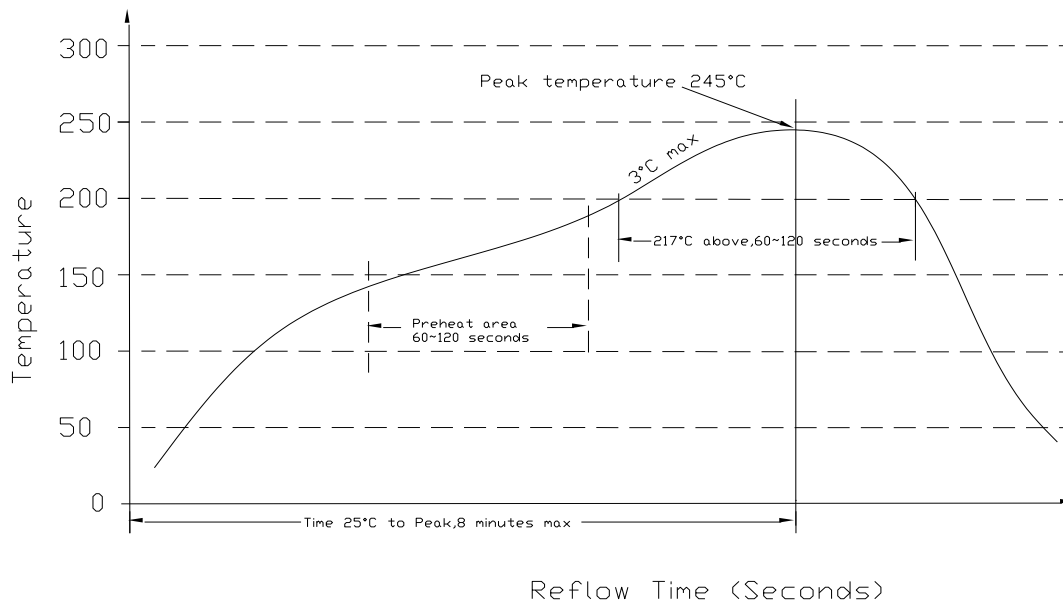
Figure 30. Soldering temperature
