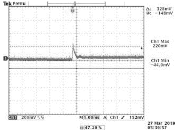
Figure 14. 75%-50% Load Transients at V_{in} = 54 V @ T_a = 25^{\circ}C
