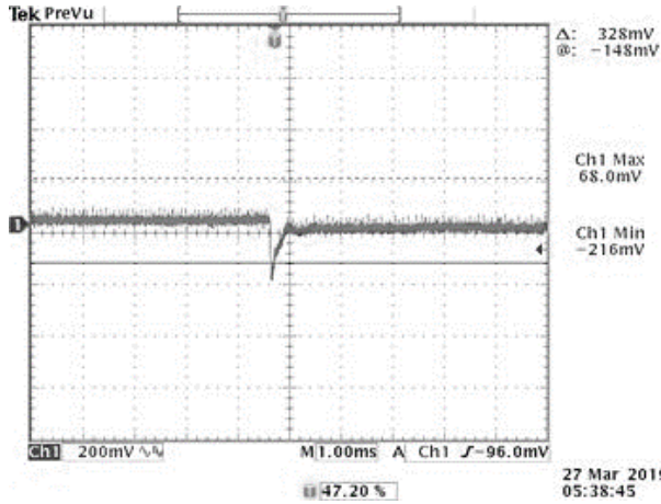
Figure 13. 50%-75% Load Transients at V_{in} = 54 V @ T_a = 25^{\circ}C
