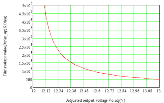
Figure 13. Trim up curve
