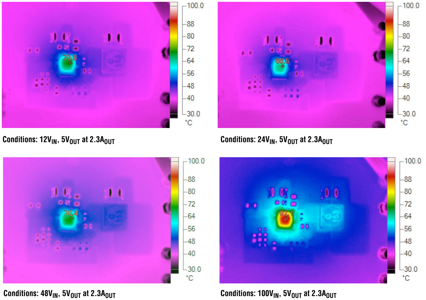
Figure 7. Thermal Plots ( T_A = 25^\circ\text{C} , without Forced Air)
