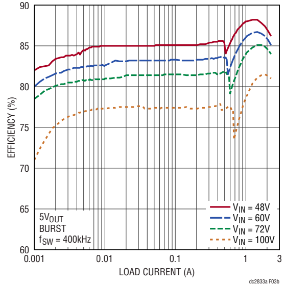
Figure 3. Efficiency at Various Input Voltages (Conditions: Burst Mode Operation)
