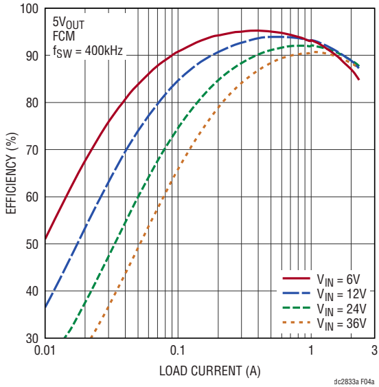
Figure 4. Efficiency at Various Input Voltages (Conditions: Forced Continuous Mode)
