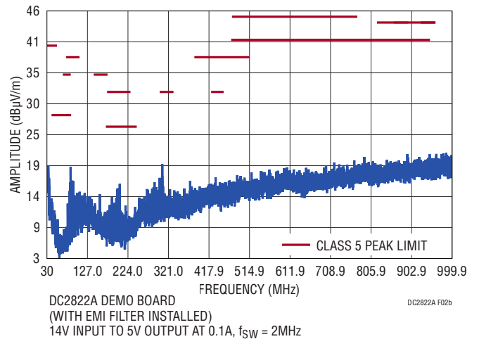
Figure 2. EMI Performance of the DC2822A. V_{IN} = 14\text{V} , I_{OUT} = 100\text{mA}
