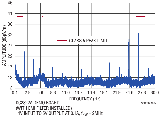
Figure 2. EMI Performance of the DC2822A. V_{IN} = 14\text{V} , I_{OUT} = 100\text{mA}
