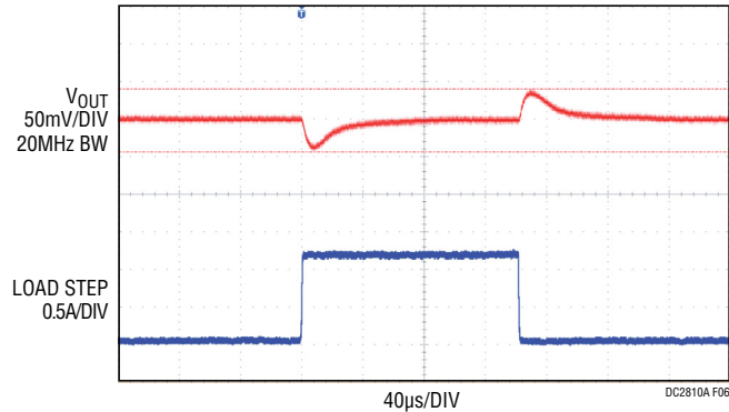
CHANNEL 1 SINGLE OUTPUT CONFIGURATION
