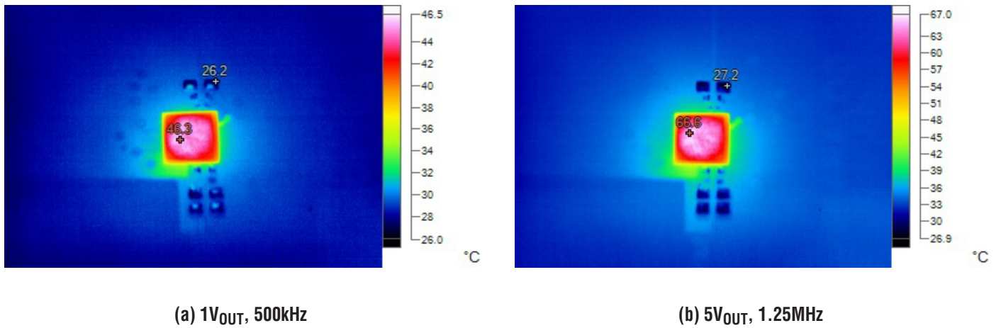
Figure 3. Measured Thermal Capture at 12V_{IN} , I_{OUT} = 8A at 25^{\circ}C Ambient with No Airflow
