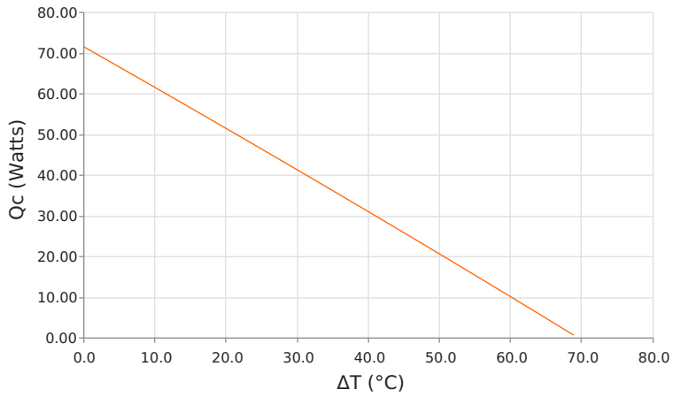
Heat Pumped at Cold Side (Qc) Thot = 27 °C | Current = 6.2 Amps
