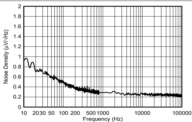
Figure 6-27. Voltage Output Noise Density
