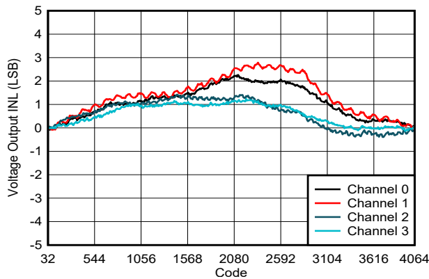
Internal reference, gain = 4 × Figure 6-4. Voltage Output INL vs Digital Input Code
