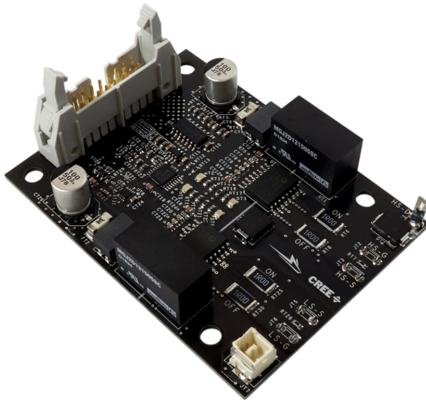
Figure 10 CGD1200HB2P-BM dual channel differential isolated gate driver
