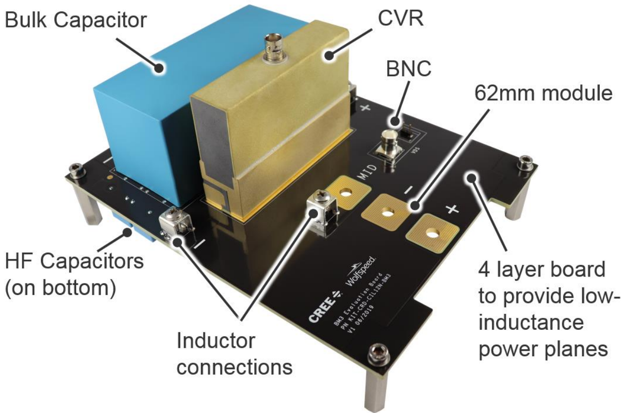
Figure 4 Evaluation Board
