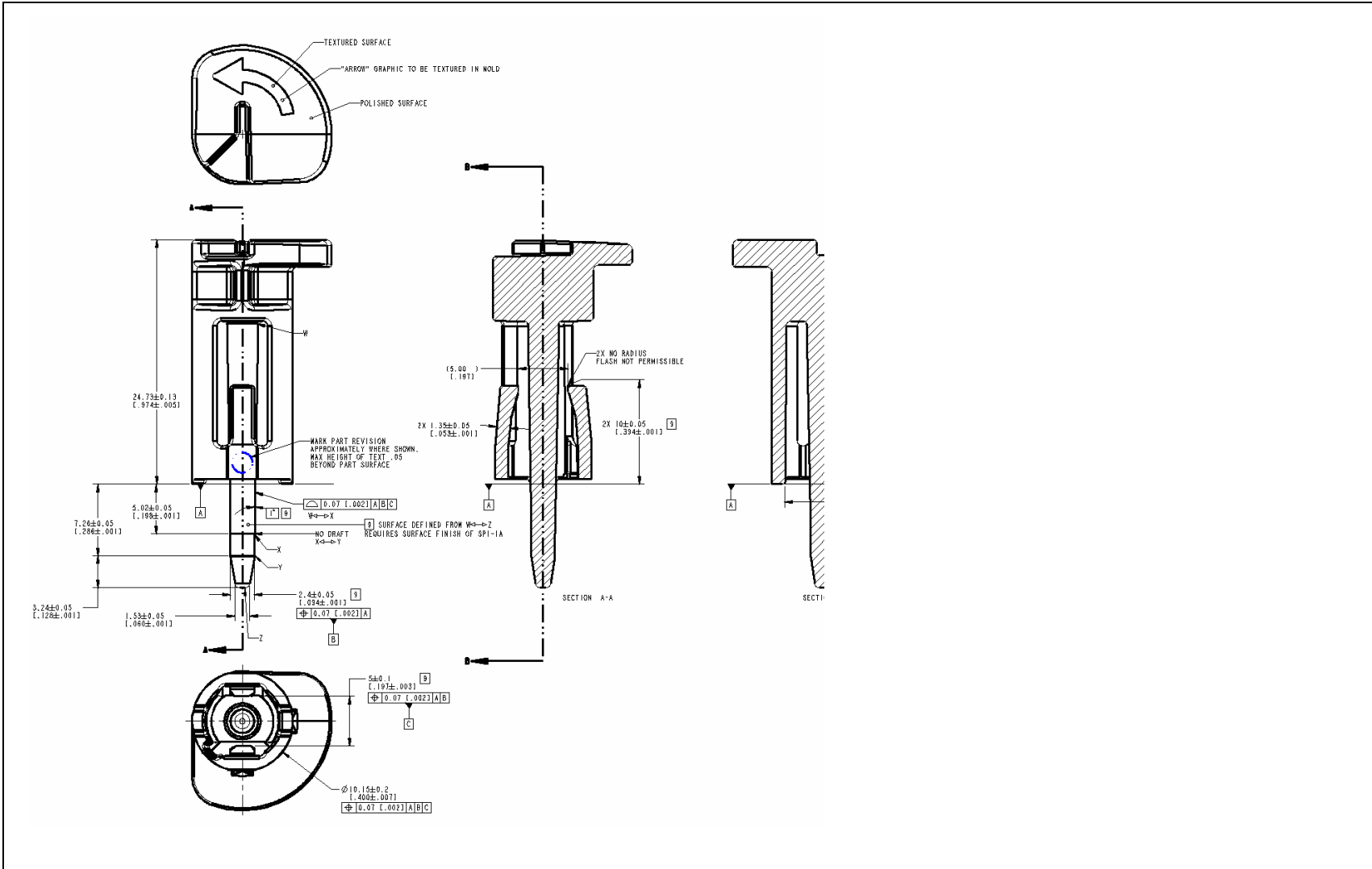
Figure 7-53. Reference Fastener - Sheet 4
