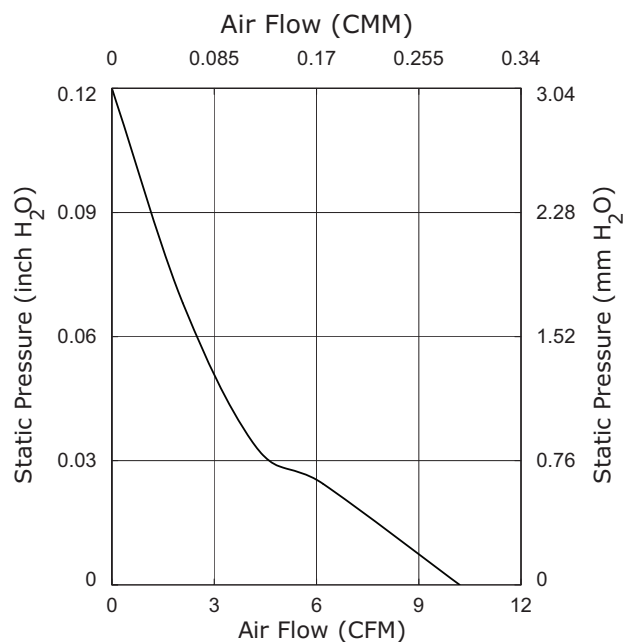
CFM-5015V-161-330
