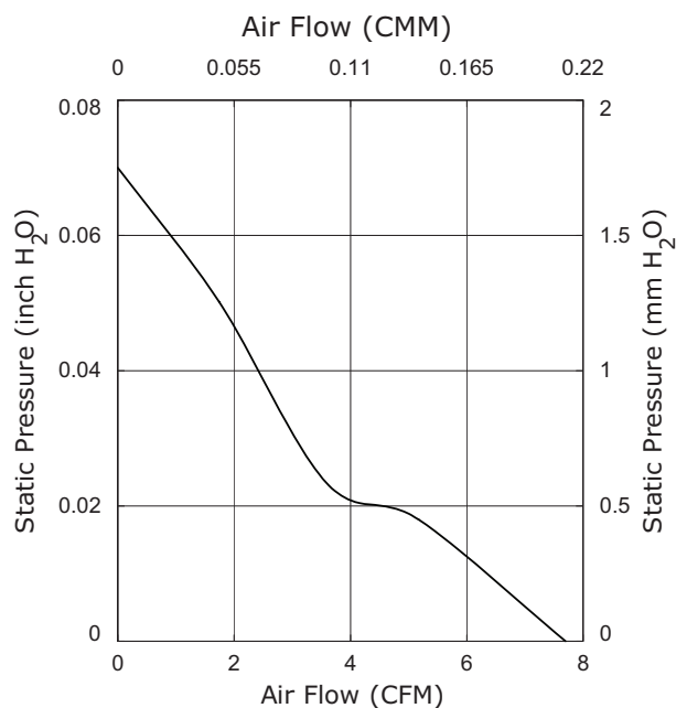
CFM-5015V-150-290
