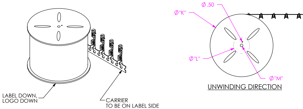
FIG 3 REEL SPECIFICATIONS
