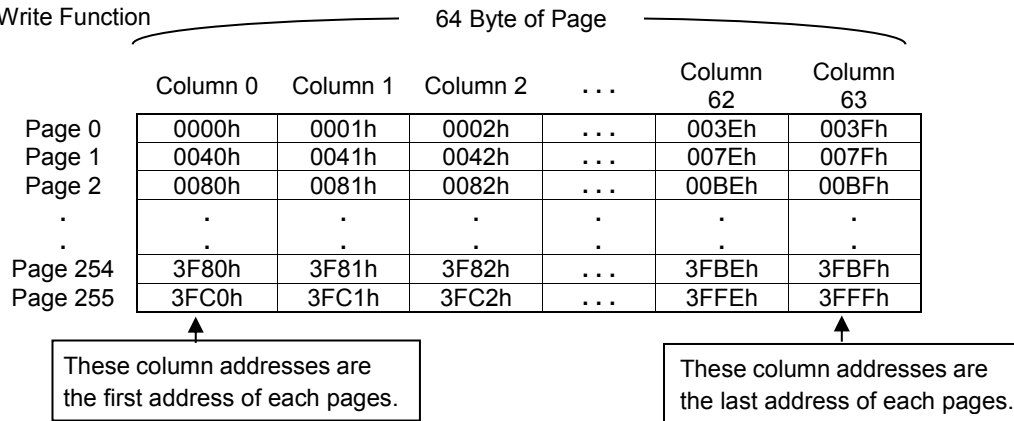
Figure 44. EEPROM physical address for Page Write command (64 Byte)
