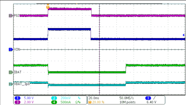
Figure 8-5. Charge Disable
