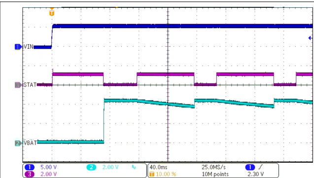
Figure 8-3. Power Up Without Battery
