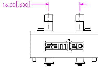
FIG 5 BE70A-S-XXXX-X-2-08-XXXX SHOWN CABLE ASSEMBLIES NOT SHOWN FOR CLARITY
