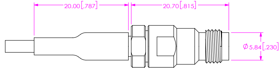
FIG 11 -18SJ SHOWN (CABLE CUT FOR CLARITY ONLY)
