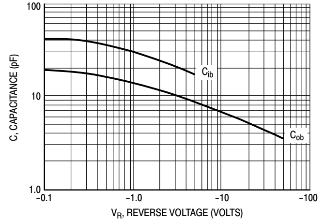
Figure 7. Capacitances
