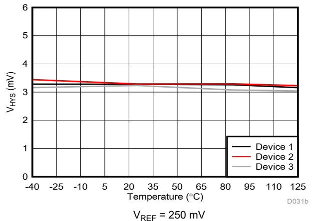
Figure 6-46. Cmp1 Trip Threshold Hysteresis vs Temperature
