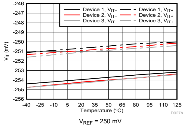
Figure 6-42. Cmp1 Trip Threshold vs Temperature
