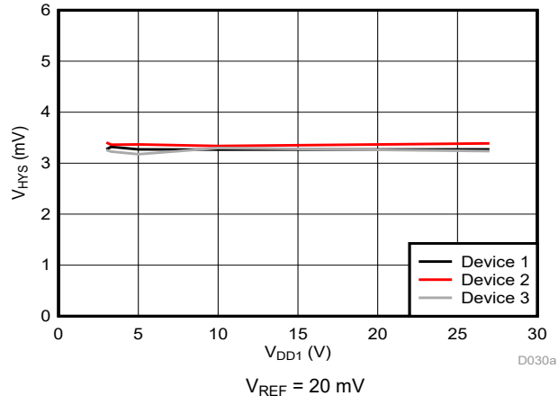
Figure 6-39. Cmp1 Trip Threshold Hysteresis vs Supply Voltage
