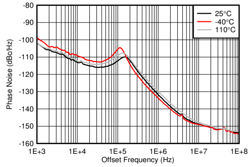
Figure 6-521. Phase Noise for 8-GHz VCO vs Offset Frequency and Temperature at f_{OUT} = 1910 \text{ MHz}
