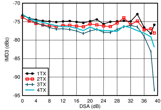
Figure 6-97. TX IMD3 vs DSA Setting at 2.6 GHz
