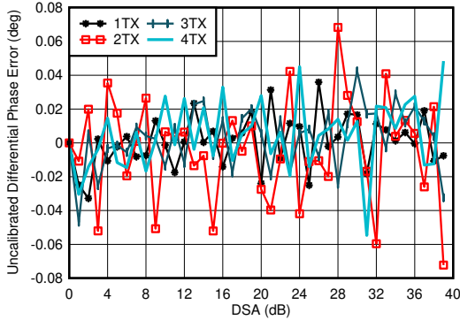
f_{\text{DAC}} = 8847.36\text{MSPS} , straight mode, matching at 2.6 GHz Differential Phase Error = \text{Phase}_{\text{OUT}}(\text{DSA Setting} - 1) - \text{Phase}_{\text{OUT}}(\text{DSA Setting})
