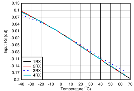
Figure 6-288. RX Input Fullscale vs Temperature and Channel at 800MHz
