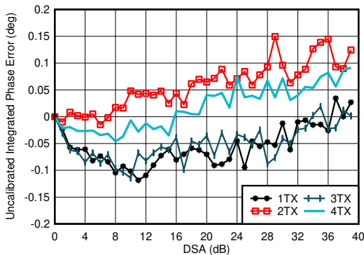
f_{\text{DAC}} = 8847.36\text{MSPS} , straight mode, matching at 2.6 GHz Integrated Phase Error = \text{Phase}(\text{DSA Setting}) - \text{Phase}(\text{DSA Setting} = 0)
