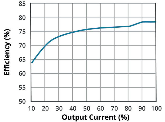
EFFICIENCY VS OUTPUT LOAD AE10-EW-S9-DIN
