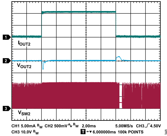
Figure 48. Buck Regulator Load Transient Response, V_{VINP} = 24\text{ V} , V_{OUT1} = 24\text{ V} , V_{OUT2} = 5\text{ V} , I_{OUT2} = 0.3\text{ mA} to 11\text{ mA} Step, T_A = 25^\circ\text{C}
