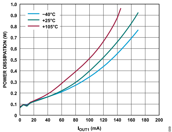
Figure 9. Power Dissipation Across Temperature, V_{VINP} = 24\text{ V} , V_{OUT1} = 24\text{ V} , V_{OUT2} = 5.0\text{ V} , I_{OUT2} = 6\text{ mA} , V_{OUT3} = -15\text{ V} , I_{OUT3} = -4\text{ mA}
