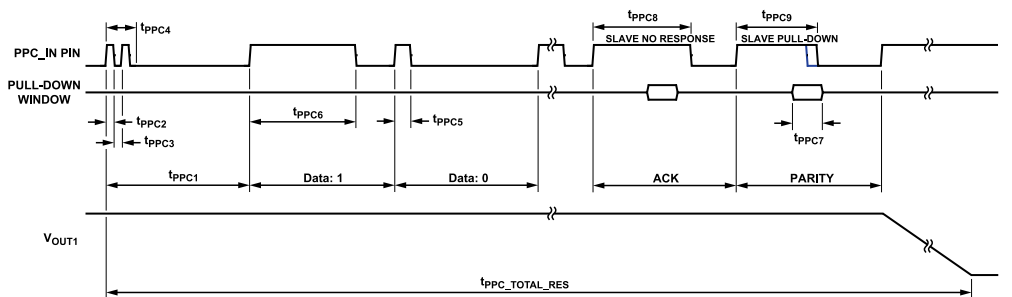
Figure 2. PPC Timing Diagram for a Complete Transmission
