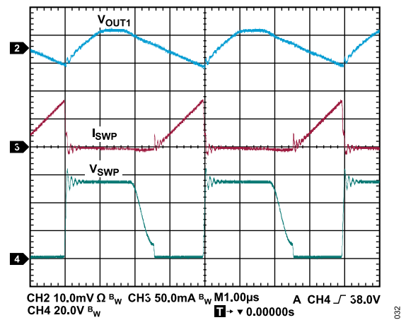
Figure 27. Flyback Regulator Discontinuous Conduction Mode Operation Showing I_{SWP} , Switch Node Voltage, and Output Ripple, T_A = 25^\circ\text{C} , V_{INP} = 24\text{ V} , V_{OUT1} = 24\text{ V} , I_{OUT1} = 20\text{ mA}
