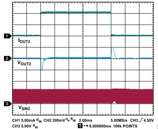
Figure 51. Buck Regulator Load Transient Response, V_{VINP} = 24\text{ V} , V_{OUT1} = 6\text{ V} , V_{OUT2} = 5\text{ V} , I_{OUT2} = 0.3\text{ mA} to 11\text{ mA} Step, T_A = 25^\circ\text{C}
