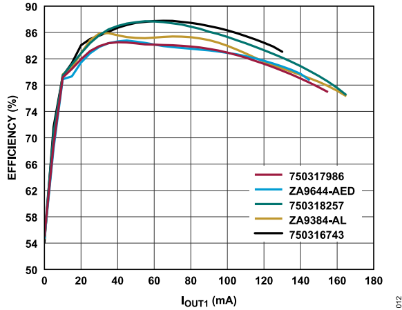
Figure 12. Overall Efficiency Using Various Transformers, T_A = 105^\circ\text{C} , V_{VINP} = 24\text{ V} , V_{OUT1} = 24\text{ V} , V_{OUT2} = 5.0\text{ V} , I_{OUT2} = 6\text{ mA} , V_{OUT3} = -15\text{ V} , I_{OUT3} = -4\text{ mA}
