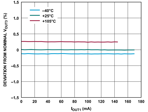
Figure 56. Inverting Regulator Cross Regulation Across Temperature, V_{VINP} = 24\text{ V} , V_{OUT3} = -15\text{ V} , I_{OUT2} = -4\text{ mA}
