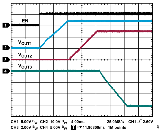
Figure 13. Power-Up Sequence, T_A = 25^\circ\text{C} , V_{VINP} = 24\text{ V} , V_{OUT1} = 24\text{ V} , I_{OUT1} = 25\text{ mA} , V_{OUT2} = 5.0\text{ V} , I_{OUT2} = 6\text{ mA} , V_{OUT3} = -15\text{ V} , I_{OUT3} = -4\text{ mA}
