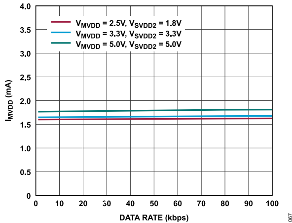
Figure 67. I_{MVDD} vs. Data Rate on All GPIO Channels at Various Supply Voltages, \overline{MSS} = High
