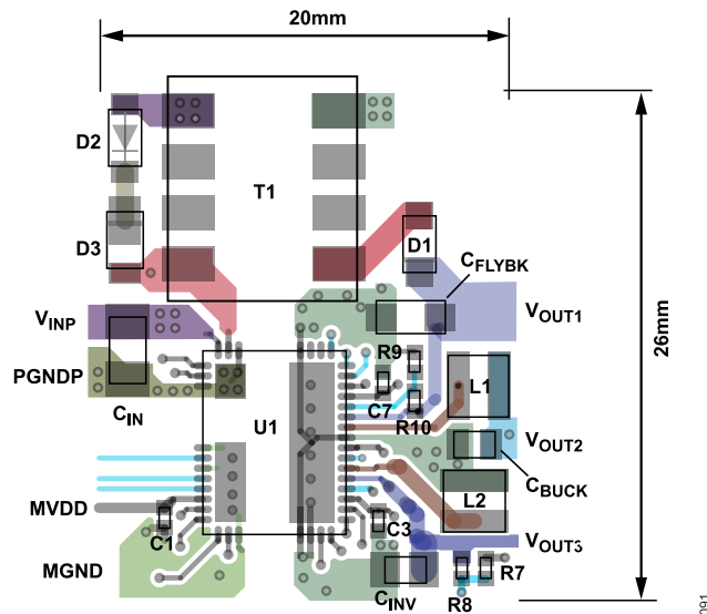
Figure 90. Suggested ADP1034 Top Layer Layout
