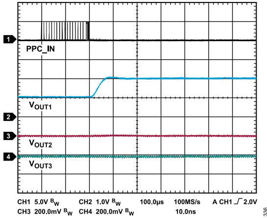
Figure 36. PPC with Step of Nine Codes, from V_{OUT1} 16\text{ V} to 17\text{ V} , V_{VINP} = 24\text{ V} , V_{OUT1} Load = 1\text{ k}\Omega , V_{OUT2} = 5.0\text{ V} , I_{OUT2} = 6\text{ mA} , V_{OUT3} = -15\text{ V} , I_{OUT3} = -4\text{ mA} , T_A = 25^\circ\text{C}
