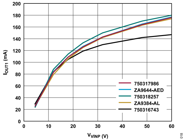
Figure 18. Flyback Regulator Maximum Output Current ( I_{OUT1} ) vs. V_{VINP} Over Various Transformers, T_A = 25^\circ\text{C} , V_{OUT1} = 24\text{ V} , Using a Zener Clamp Circuit, Based on Target of 70% I_{LIM} (FLYBACK)
