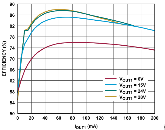
Figure 7. Overall Efficiency at Various V_{OUT1} Output Voltages, T_A = 25^\circ\text{C} , V_{VINP} = 24\text{ V} , V_{OUT2} = 5.0\text{ V} , I_{OUT2} = 6\text{ mA} , V_{OUT3} = -15\text{ V} , I_{OUT3} = -4\text{ mA}
