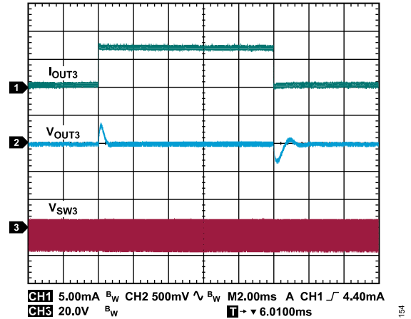
Figure 62. Inverting Regulator Load Transient Response, V_{VINP} = 24\text{ V} , V_{OUT1} = 24\text{ V} , I_{OUT1} = 26\text{ mA} , V_{OUT2} = 5\text{ V} , I_{OUT2} = 11\text{ mA} , V_{OUT3} = -15\text{ V} , I_{OUT3} = -0.3\text{ mA} to -7\text{ mA} Step, T_A = 25^\circ\text{C}
