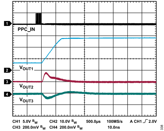
Figure 38. PPC Full Output Range Step, from V_{OUT1} = 6\text{ V} to 28\text{ V} , V_{VINP} = 24\text{ V} , V_{OUT1} Load = 250\ \Omega , V_{OUT2} = 5.0\text{ V} , I_{OUT2} = 6\text{ mA} , V_{OUT3} = -15\text{ V} , I_{OUT3} = -4\text{ mA} , T_A = 25^\circ\text{C}
