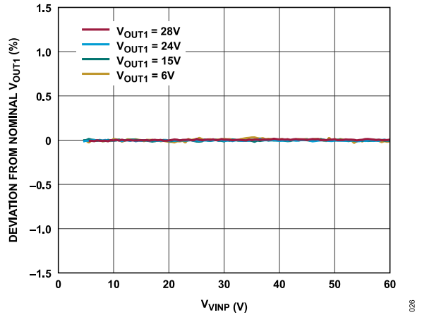
Figure 26. Flyback Regulator Line Regulation at Various Output Voltages, T_A = 25^\circ\text{C} , I_{OUT1} = 25\text{ mA} , Nominal = V_{OUT1} with V_{INP} = 24\text{ V}
