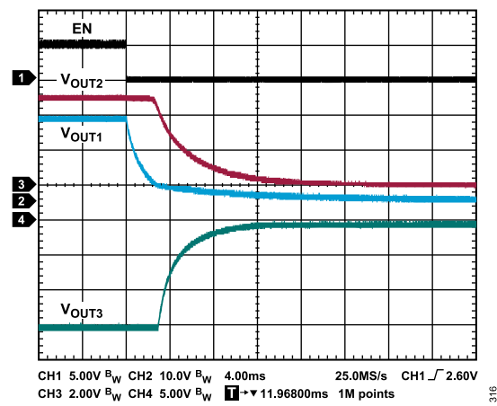
Figure 16. Shutdown Sequence, T_A = 25^\circ\text{C} , V_{VINP} = 24\text{ V} , V_{OUT1} = 24\text{ V} , I_{OUT1} = 25\text{ mA} , V_{OUT2} = 5.0\text{ V} , I_{OUT2} = 6\text{ mA} , V_{OUT3} = -15\text{ V} , I_{OUT3} = -4\text{ mA}
