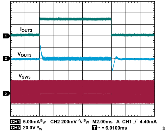
Figure 59. Inverting Regulator Load Transient Response, V_{VINP} = 24\text{ V} , V_{OUT1} = 24\text{ V} , I_{OUT1} = 0\text{ mA} , V_{OUT2} = 5\text{ V} , I_{OUT2} = 0\text{ mA} , V_{OUT3} = -15\text{ V} , I_{OUT3} = -0.3\text{ mA} to -7\text{ mA} Step, T_A = 25^\circ\text{C}
