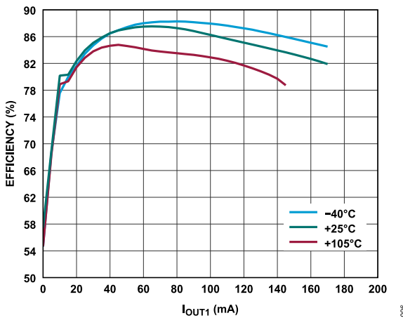
Figure 6. Overall Efficiency Across Temperature, V_{VINP} = 24\text{ V} , V_{OUT1} = 24\text{ V} , V_{OUT2} = 5.0\text{ V} , I_{OUT2} = 6\text{ mA} , V_{OUT3} = -15\text{ V} , I_{OUT3} = -4\text{ mA}
