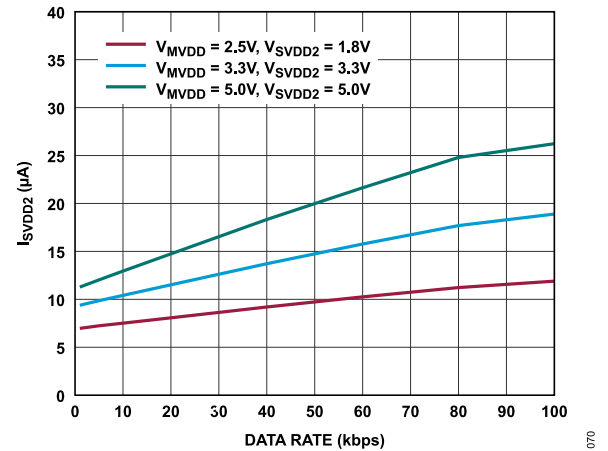
Figure 70. I_{SVDD2} vs. Data Rate on All GPIO Channels at Various Supply Voltages, \overline{MSS} = High
