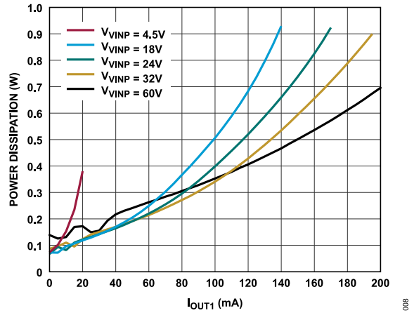
Figure 8. Power Dissipation at Various Input Voltages, T_A = 25^\circ\text{C} , V_{OUT1} = 24\text{ V} , V_{OUT2} = 5.0\text{ V} , I_{OUT2} = 6\text{ mA} , V_{OUT3} = -15\text{ V} , I_{OUT3} = -4\text{ mA}
