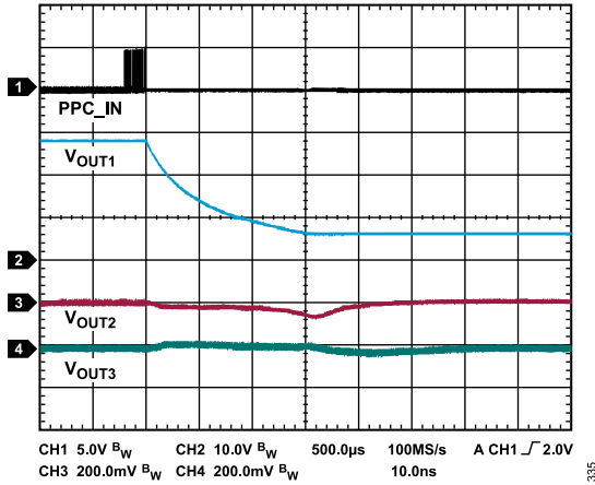
Figure 35. PPC Full Output Range Step, from V_{OUT1} = 28\text{ V} to 6\text{ V} , V_{VINP} = 24\text{ V} , V_{OUT1} Load = 250\ \Omega , V_{OUT2} = 5.0\text{ V} , I_{OUT2} = 6\text{ mA} , V_{OUT3} = -15\text{ V} , I_{OUT3} = -4\text{ mA} , T_A = 25^\circ\text{C}
