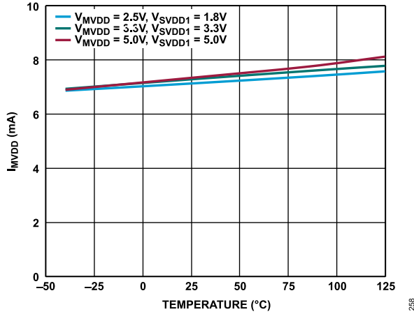
Figure 65. I_{MVDD} vs. Temperature at Various Supply Voltages, \overline{MSS} = Low , Data Rate = 10 Mbps on All SPI Channels
