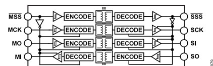
Figure 79. iCoupler Gating
