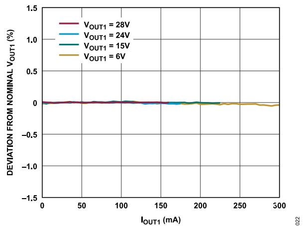
Figure 22. Flyback Regulator Load Regulation at Various Output Voltages, T_A = 25^\circ\text{C} , V_{VINP} = 24\text{ V} , Nominal = V_{OUT1} at 25 mA Load
