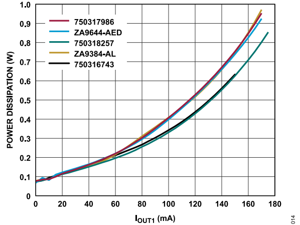
Figure 14. Power Dissipation Using Various Transformers, T_A = 25^\circ\text{C} , V_{VINP} = 24\text{ V} , V_{OUT1} = 24\text{ V} , V_{OUT2} = 5.0\text{ V} , I_{OUT2} = 6\text{ mA} , V_{OUT3} = -15\text{ V} , I_{OUT3} = -4\text{ mA}
