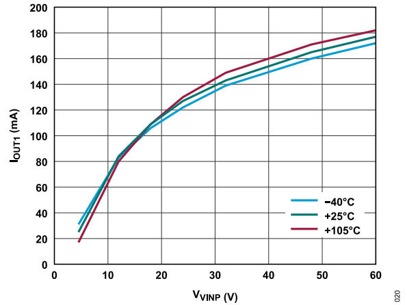
Figure 20. Flyback Regulator Maximum Output Current ( I_{OUT1} ) vs. V_{VINP} Across Temperature, V_{OUT1} = 24\text{ V} , Using a Coilcraft ZA9644-AED Transformer and a Zener Clamp Circuit, Based on Target of 70% I_{LIM} (FLYBACK)
