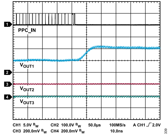
Figure 39. PPC with Step of One Code, V_{OUT1} = 10\text{ V} + 1\text{ LSB} ( 0.111\text{ V} ), V_{VINP} = 24\text{ V} , V_{OUT1} Load = 1\text{ k}\Omega , V_{OUT2} = 5.0\text{ V} , I_{OUT2} = 6\text{ mA} , V_{OUT3} = -15\text{ V} , I_{OUT3} = -4\text{ mA} , T_A = 25^\circ\text{C}
