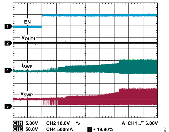
Figure 28. Flyback Regulator Short-Circuit Current Limit During Startup, V_{INP} = 24\text{ V} , V_{OUT1} = \text{SGND2} , T_A = 25^\circ\text{C}
