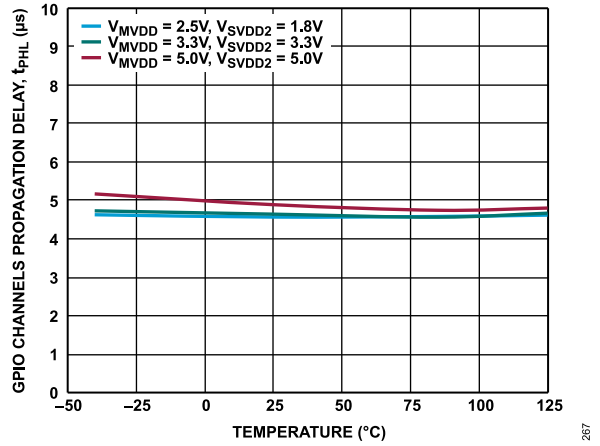
Figure 74. GPIO Channels Propagation Delay ( t_{PHL} ) vs. Temperature at Various Supply Voltages
