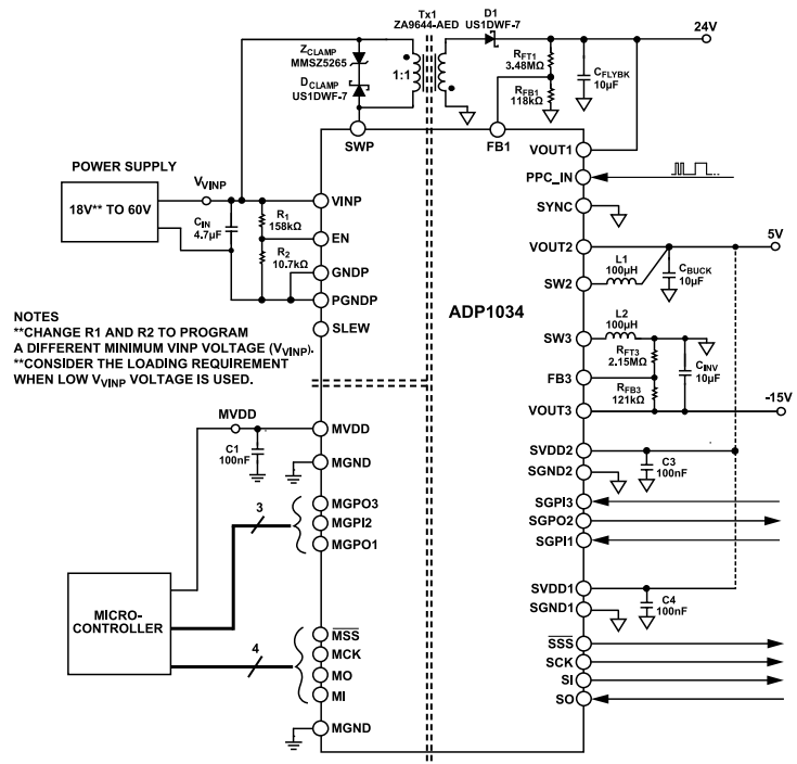
Figure 89. Detailed Typical Application Circuit
