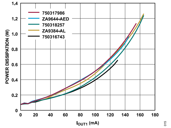
Figure 15. Power Dissipation Using Various Transformers, T_A = 105^\circ\text{C} , V_{VINP} = 24\text{ V} , V_{OUT1} = 24\text{ V} , V_{OUT2} = 5.0\text{ V} , I_{OUT2} = 6\text{ mA} , V_{OUT3} = -15\text{ V} , I_{OUT3} = -4\text{ mA}
