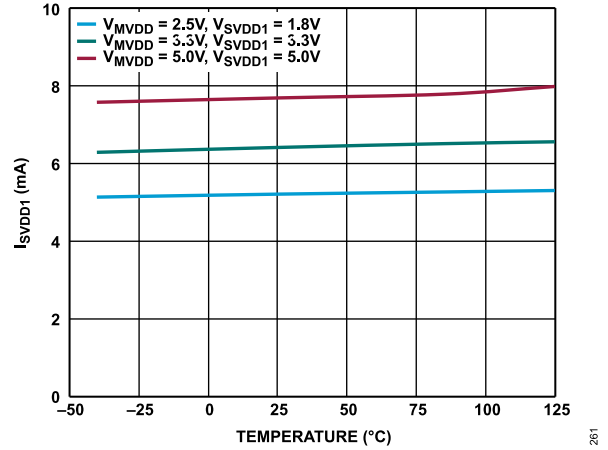
Figure 68. I_{SVDD1} vs. Temperature at Various Supply Voltages, \overline{SSS} = Low , Data Rate = 10 Mbps on All SPI Channels
