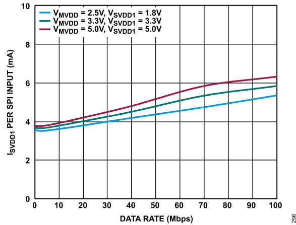
Figure 63. I_{SVDD1} Supply Current ( I_{SVDD1} ) per SPI Input vs. Data Rate at Various Supply Voltages, \overline{SSS} = \text{Low} , Clock Signal Applied on Single SPI Channel, Other Input Channels Tied Low
