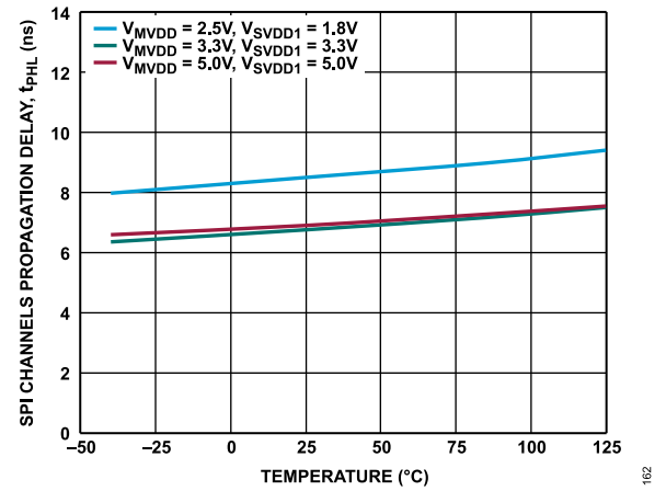
Figure 69. SPI Channels Propagation Delay ( t_{PHL} ) vs. Temperature at Various Supply Voltages
