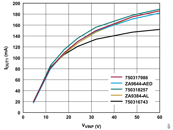
Figure 21. Flyback Regulator Maximum Output Current ( I_{OUT1} ) vs. V_{VINP} Over Various Transformers, T_A = 105^\circ\text{C} , V_{OUT1} = 24\text{ V} , Using a Zener Clamp Circuit, Based on Target of 70% I_{LIM} (FLYBACK)
