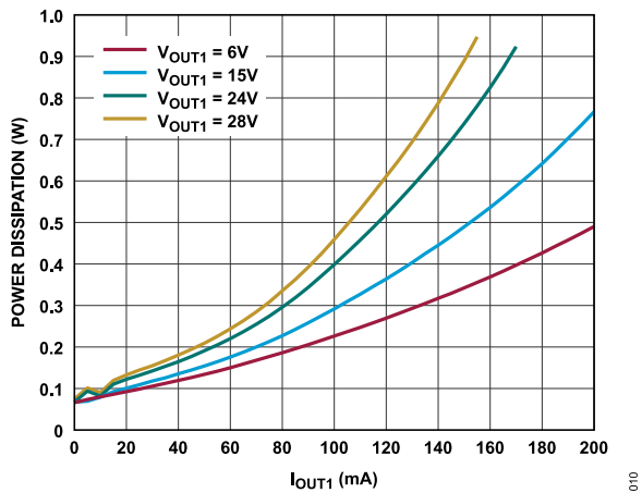
Figure 10. Power Dissipation at Various V_{OUT1} Output Voltages, T_A = 25^\circ\text{C} , V_{VINP} = 24\text{ V} , V_{OUT2} = 5.0\text{ V} , I_{OUT2} = 6\text{ mA} , V_{OUT3} = -15\text{ V} , I_{OUT3} = -4\text{ mA}
