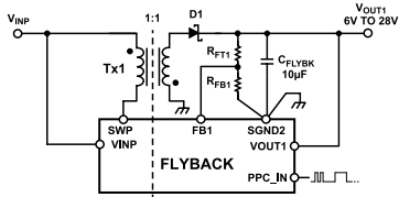
Figure 82. Flyback Regulator Output Voltage Setting
