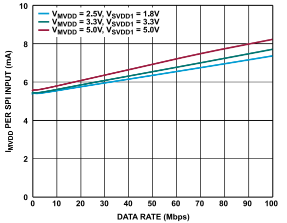
Figure 60. I_{MVDD} Supply Current ( I_{MVDD} ) per SPI Input vs. Data Rate at Various Supply Voltages, \overline{MSS} = \text{Low} , Clock Signal Applied on Single SPI Channel, Other Input Channels Tied Low
