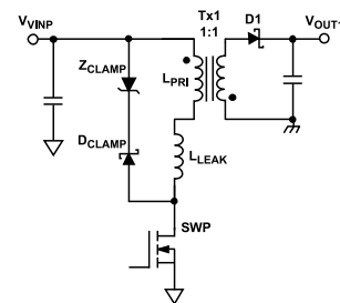
Figure 87. Diode, Zener Diode Clamp
