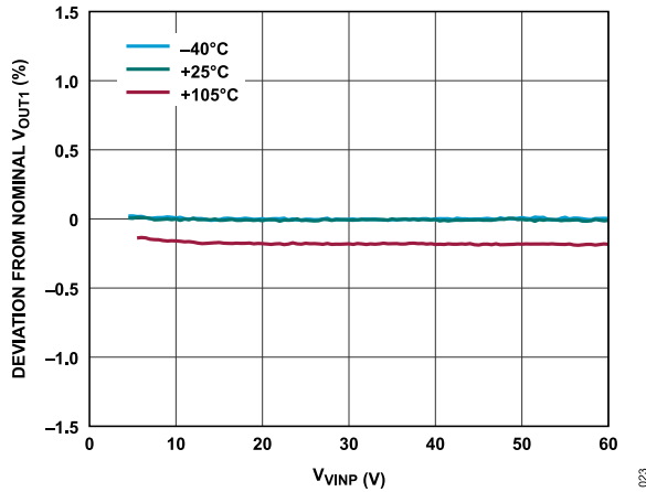
Figure 23. Flyback Regulator Line Regulation Across Temperature, V_{OUT1} = 24\text{ V} , I_{OUT1} = 25\text{ mA} , Nominal = V_{OUT1} with V_{INP} = 24\text{ V}
