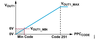
Figure 83. V_{OUT1} Output vs. PPC_{CODE}
