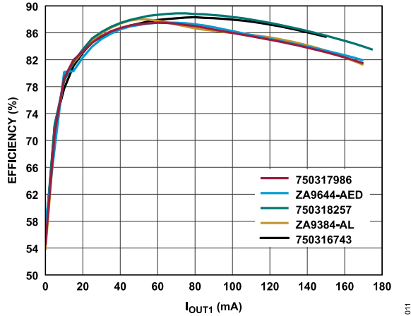
Figure 11. Overall Efficiency Using Various Transformers, T_A = 25^\circ\text{C} , V_{VINP} = 24\text{ V} , V_{OUT1} = 24\text{ V} , V_{OUT2} = 5.0\text{ V} , I_{OUT2} = 6\text{ mA} , V_{OUT3} = -15\text{ V} , I_{OUT3} = -4\text{ mA}
