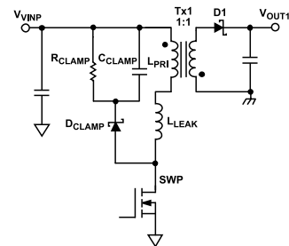
Figure 86. Resistor, Capacitor, Diode Clamp
