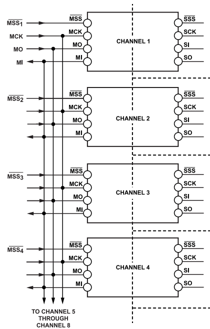
Figure 81. Multichannel SPI Muxing Scheme
