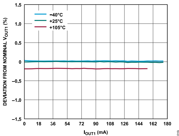
Figure 19. Flyback Regulator Load Regulation Across Temperature, V_{VINP} = 24\text{ V} , V_{OUT1} = 24\text{ V} , Nominal = V_{OUT1} at 25 mA Load
