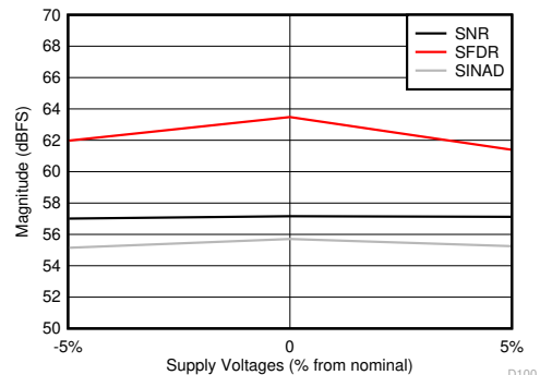
Figure 7-60. SNR, SFDR and SINAD vs Supply Voltage All supplies changed together, high power mode
