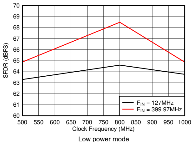
Figure 7-29. SFDR vs Sample Rate
