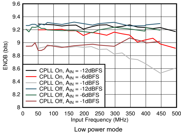
Figure 7-57. ENOB vs A_{IN} and C-PLL
