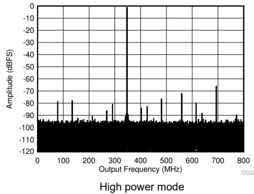
High power mode Figure 7-4. Single Tone FFT at 347 MHz and -1 dBFS
