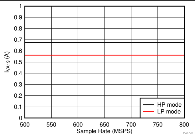
Figure 7-78. Quad Channel, I_{VA19} vs F_S Independent of JMODE
