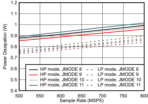
Figure 7-103. Single Channel, Power Dissipation vs F_S for JMODES 8 - 11
