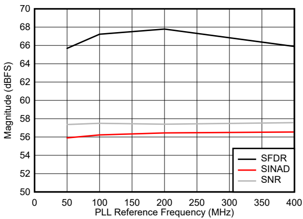
Figure 7-42. SNR, SFDR and SINAD vs Reference Frequency with PLL on
