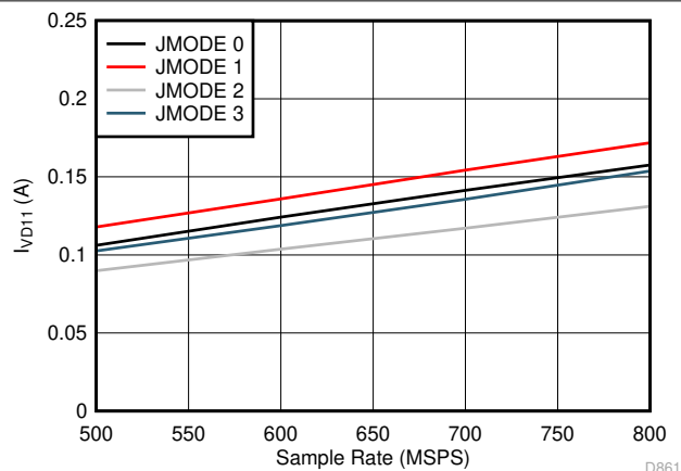
Figure 7-107. Single Channel, I_{VD11} vs F_S for JMODES 0 - 3
