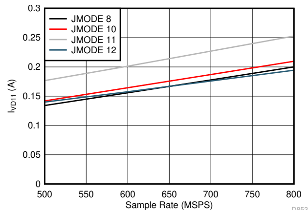
Figure 7-96. Dual Channel, I_{VD11} vs F_S for JMODES 8 - 12
