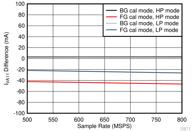
Figure 7-86. Quad Channel, I_{VA11} vs F_S over Modes
