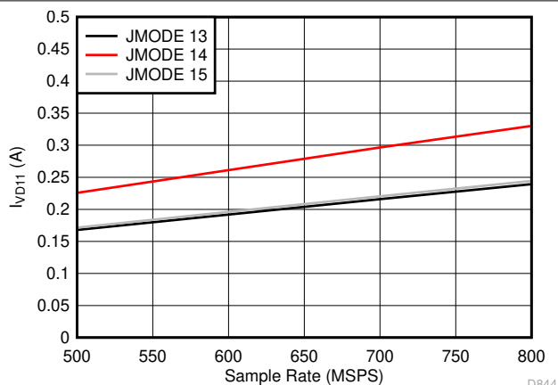
Independent of Power Mode Figure 7-83. Quad Channel, I_{VDD11} vs F_S for JMODES 13-15
