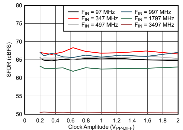
Figure 7-41. SFDR vs Clock Amplitude
