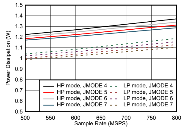
Figure 7-89. Dual Channel, Power Dissipation vs F_S for JMODES 4 - 7
