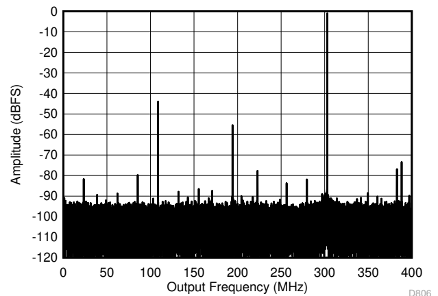
Figure 7-12. Single Tone FFT at 2097 MHz and -1dBFS Low Power Mode
