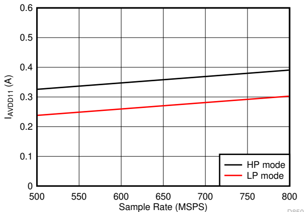
Figure 7-93. Dual Channel, I_{VA11} vs F_S Independent of JMODE
