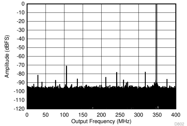
Figure 7-10. Single Tone FFT at 347 MHz and -1dBFS Low Power Mode
