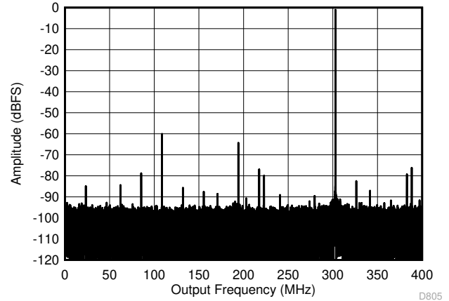
Figure 7-8. Single Tone FFT at 2097 MHz and -1dBFS
