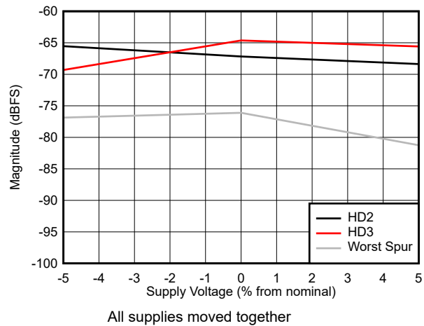
Figure 7-39. HD2, HD3 and worst non-HD vs Supply Voltage
