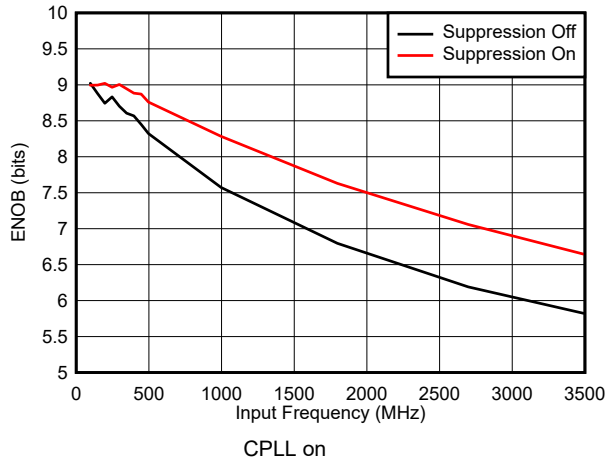
Figure 7-37. ENOB vs Input Frequency and Suppression
