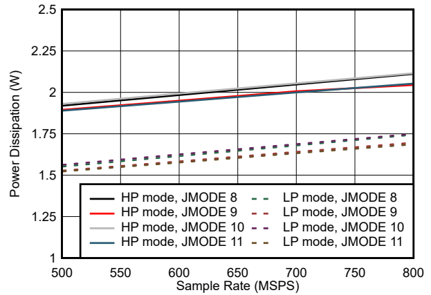
Figure 7-76. Quad Channel, Power Dissipation vs F_S for JMODES 8 - 11
