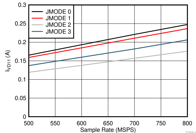
Figure 7-94. Dual Channel, I_{VD11} vs F_S for JMODES 0 - 3
