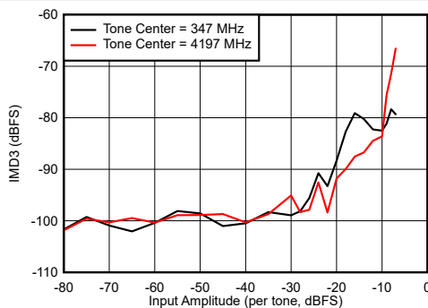
Figure 7-107. Dual Channel Mode: IMD3 vs Input Amplitude
