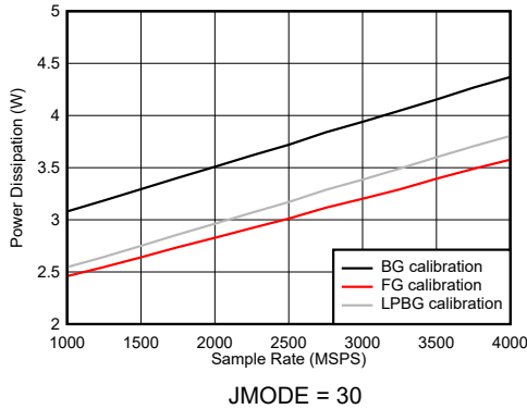
Figure 7-124. DES Mode: Power Dissipation vs Sample Rate
