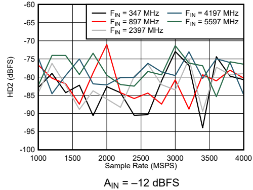
Figure 7-50. Dual Channel Mode: HD2 vs Sample Rate and Input Frequency
