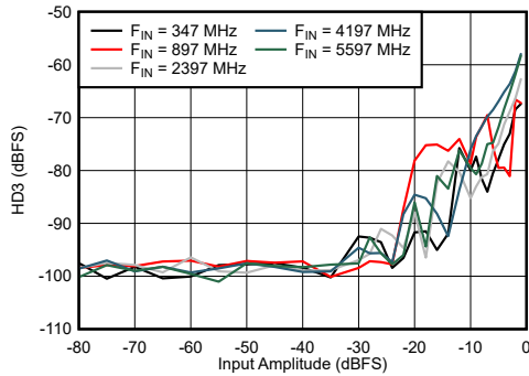
Figure 7-61. DES Mode: HD3 vs Input Amplitude and Frequency
