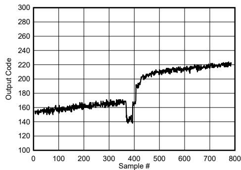
Figure 7-140. Background Calibration Core Transition (AC Signal Zoomed)
