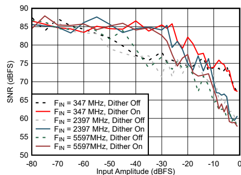
Figure 7-58. DES Mode: SFDR vs Input Amplitude and Dither
