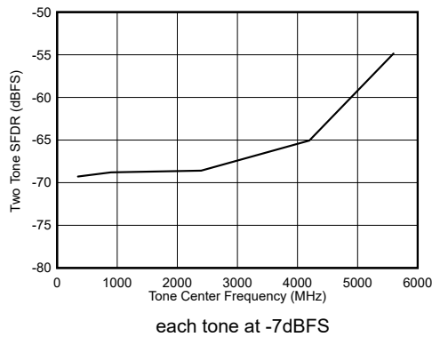
Figure 7-111. Dual Channel Mode: Two Tone SFDR vs Input Frequency
