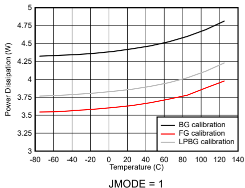
Figure 7-136. DES Mode: Power Dissipation vs Temperature
