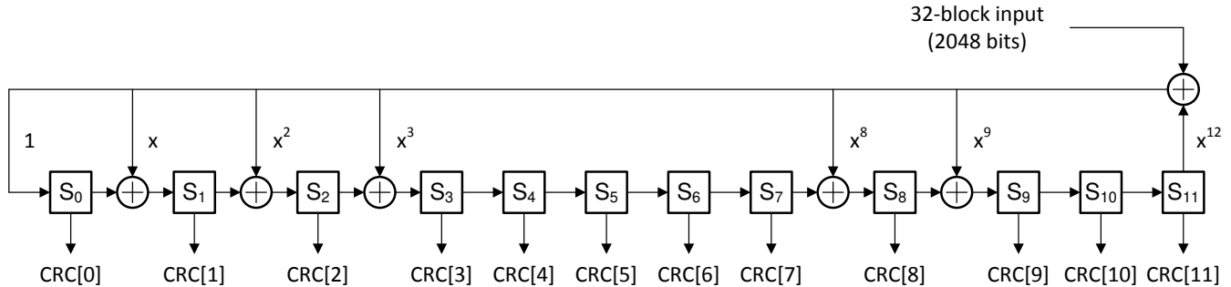
Figure 8-21. CRC-12 Parity Bit Generator
