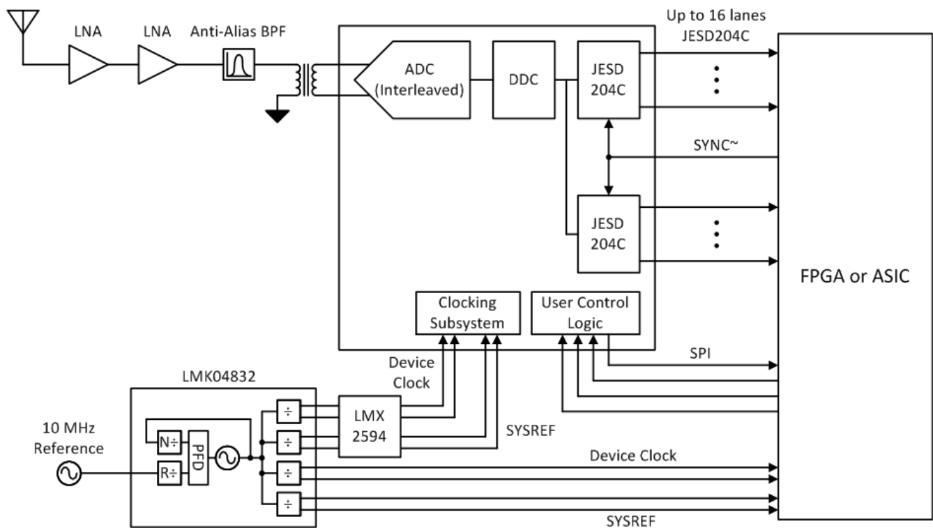
Figure 9-1. Typical Configuration for Wideband RF Sampling
