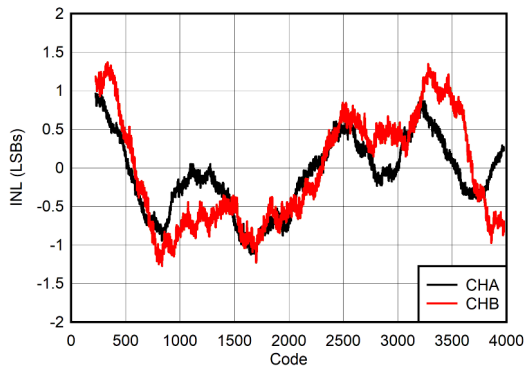
Figure 7-7. INL vs ADC Code
