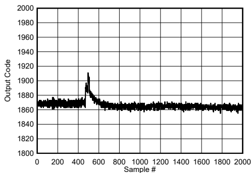
Figure 7-138. Background Calibration Core Transition (DC Offset Signal)
