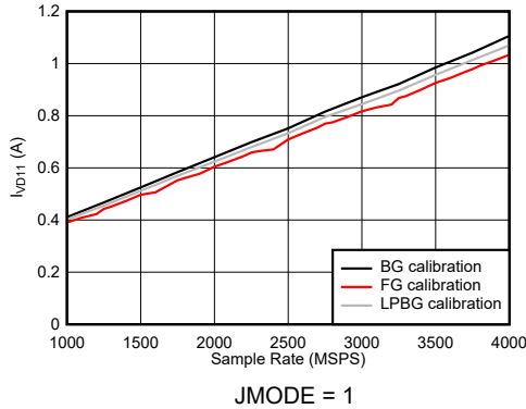
Figure 7-118. DES Mode: I_{VD11} vs Sample Rate
