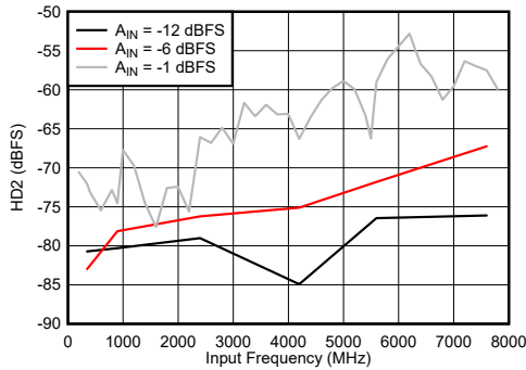
Figure 7-85. Dual Channel Mode: HD2 vs Input Frequency
