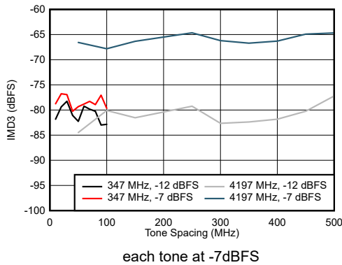
Figure 7-109. Dual Channel Mode: IMD3 vs Tone Spacing
