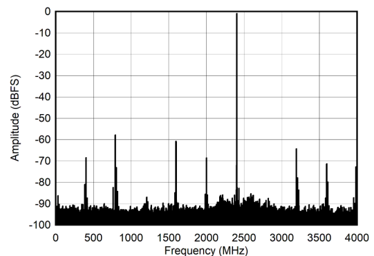
Figure 7-12. DES Mode: Single Tone FFT at 5597 MHz
