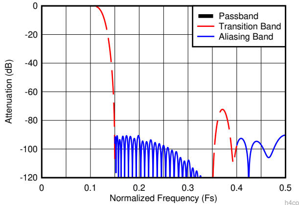
Figure 8-11. Decimate-by-4 Composite Response
