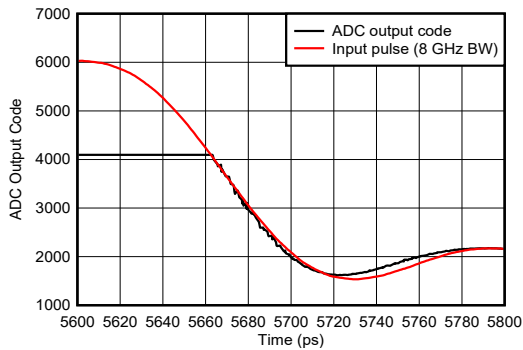
Figure 7-142. Pulse Overdrive Recovery Zoomed
