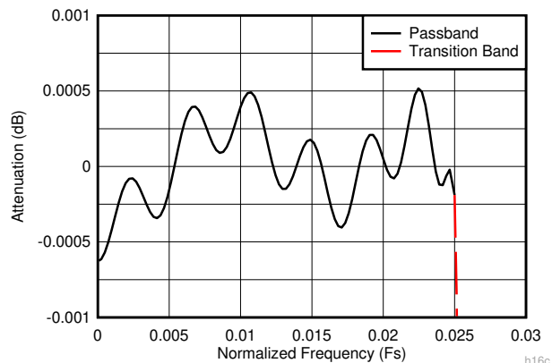
Figure 8-16. Decimate-by-16 Composite Zoomed Pass-Band Response
