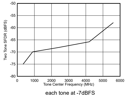
Figure 7-110. DES Mode: Two Tone SFDR vs Input Frequency
