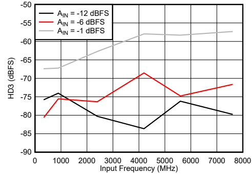
Figure 7-80. DES Mode: HD3 vs Input Frequency
