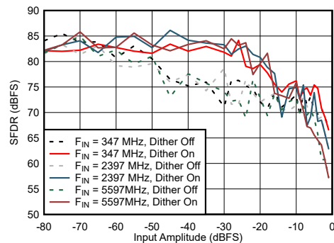
Figure 7-70. Dual Channel Mode: SFDR vs Input Amplitude and Dither
