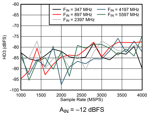
Figure 7-53. Dual Channel Mode: HD3 vs Sample Rate and Input Frequency
