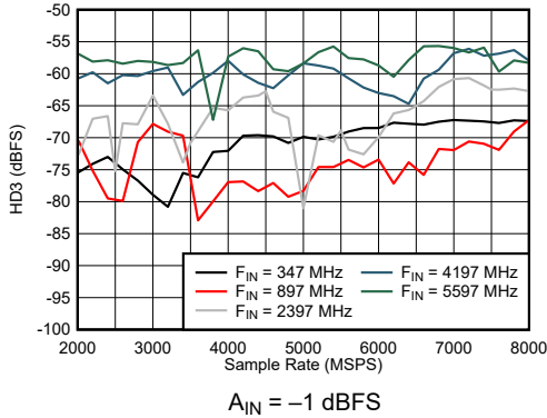
Figure 7-37. DES Mode: HD3 vs Sample Rate and Input Frequency
