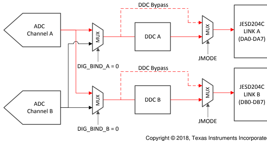
Figure 8-24. Dual DDC Mode or Redundant Data Mode for Channel A
