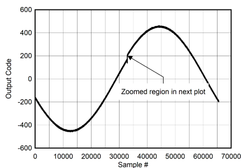
Figure 7-139. Background Calibration Core Transition (AC Signal)
