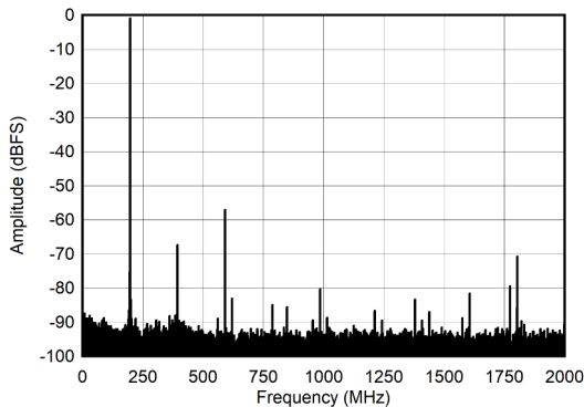
Figure 7-21. Dual Channel Mode: Single Tone FFT at 4197 MHz
