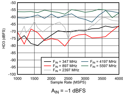
Figure 7-51. Dual Channel Mode: HD3 vs Sample Rate and Input Frequency
