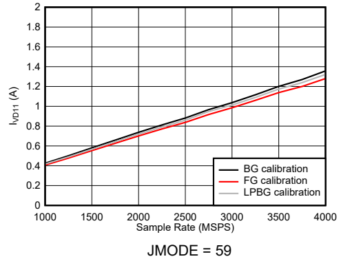
Figure 7-131. Dual Channel Mode: I_{VD11} vs Sample Rate
