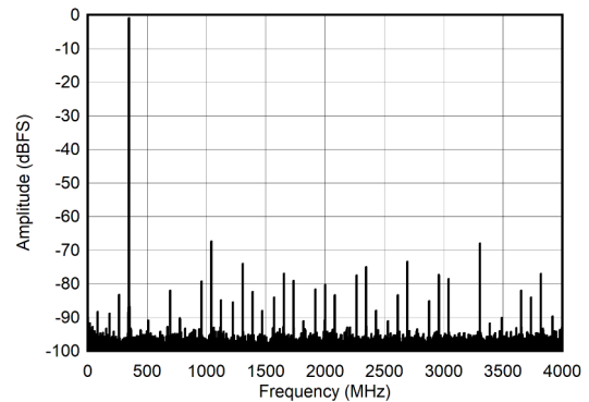
Figure 7-8. DES Mode: Single Tone FFT at 347 MHz
