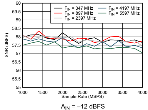
Figure 7-44. Dual Channel Mode: SNR vs Sample Rate and Input Frequency
