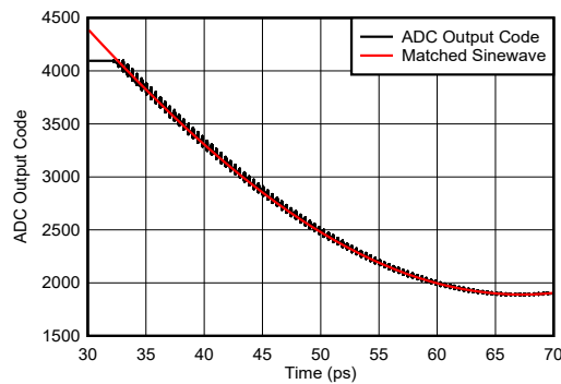
Figure 7-144. Sinewave Overdrive Recovery
