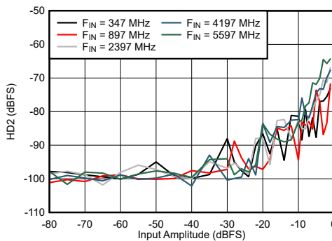
Figure 7-59. DES Mode: HD2 vs Input Amplitude and Frequency
