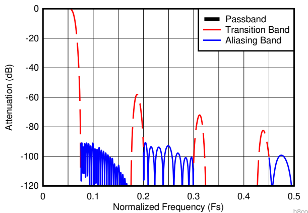
Figure 8-13. Decimate-by-8 Composite Response
