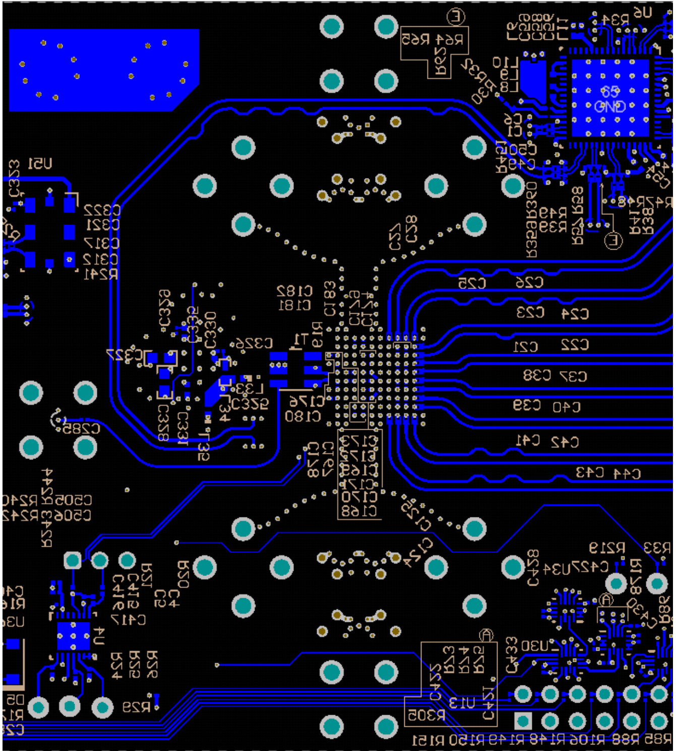
Figure 11-3. Bottom Layer Routing: Additional CLK Routing, DA4-7, DB4-7
