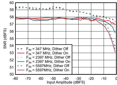
Figure 7-56. DES Mode: SNR vs Input Amplitude and Dither
