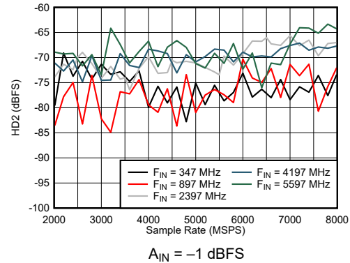
Figure 7-34. DES Mode: HD2 vs Sample Rate and Input Frequency
