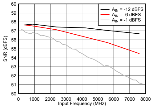
Figure 7-83. Dual Channel Mode: SNR vs Input Frequency
