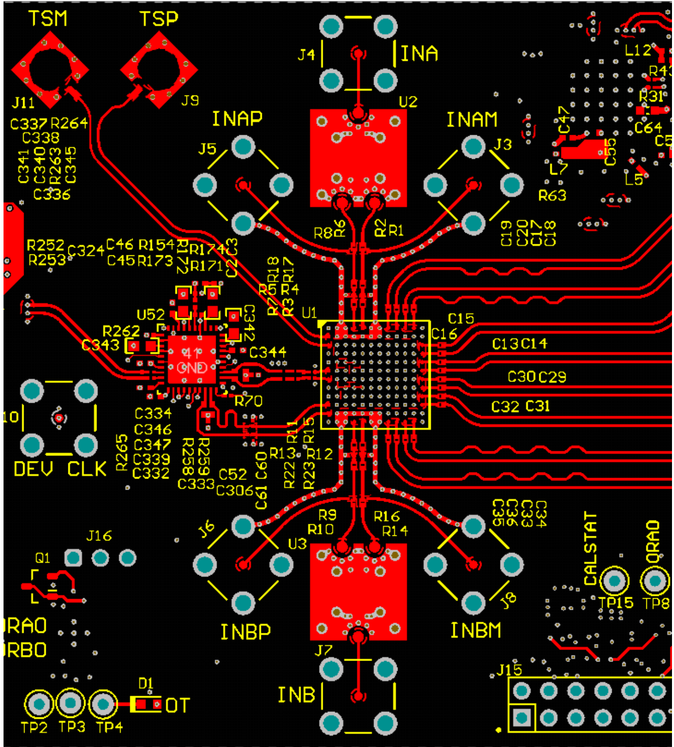
Figure 11-1. Top Layer Routing: Analog Inputs, CLK and SYSREF, DA0-3, DB0-3
