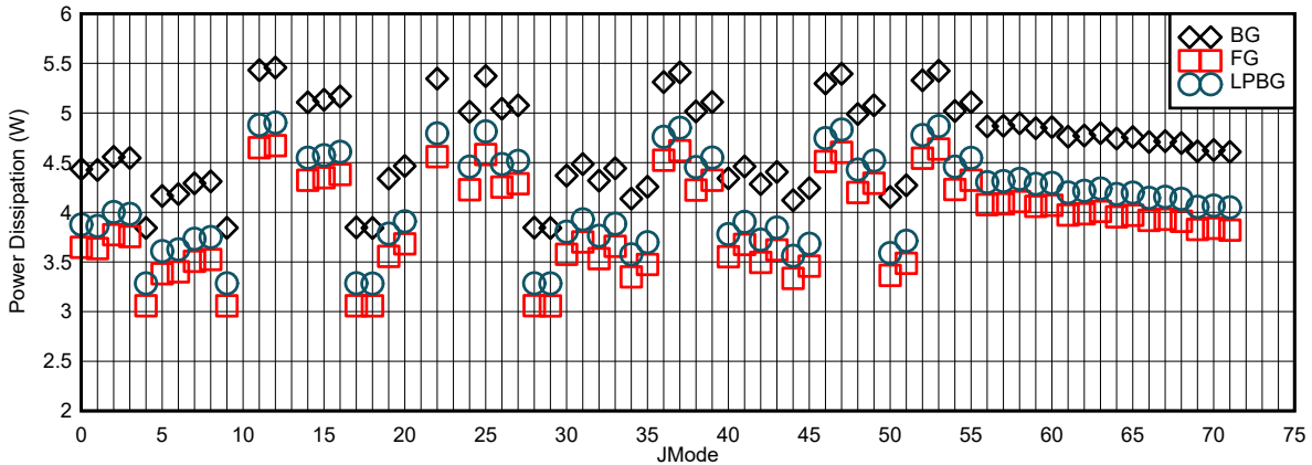
Figure 7-114. Power Dissipation vs JMODE at F_{\text{CLK}} = 4\text{ GHz}
