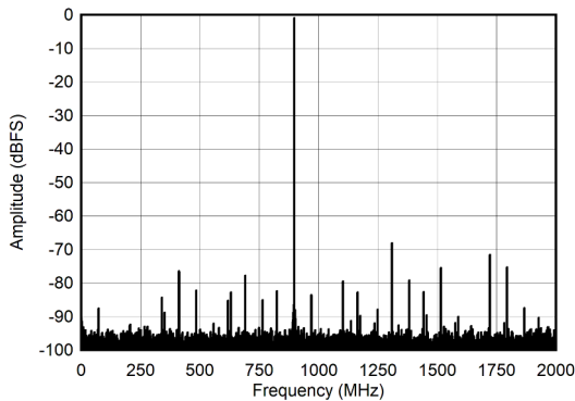
Figure 7-19. Dual Channel Mode: Single Tone FFT at 897 MHz
