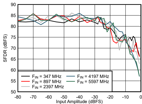
Figure 7-69. Dual Channel Mode: SFDR vs Input Amplitude and Frequency
