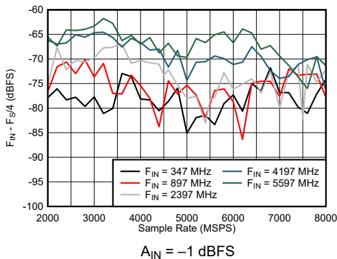
Figure 7-41. DES Mode: F_{IN} \pm F_s/4 vs Sample Rate and Input Frequency
