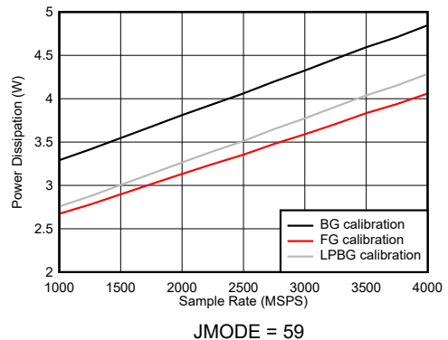
Figure 7-135. Dual Channel Mode: Power Dissipation vs Sample Rate
