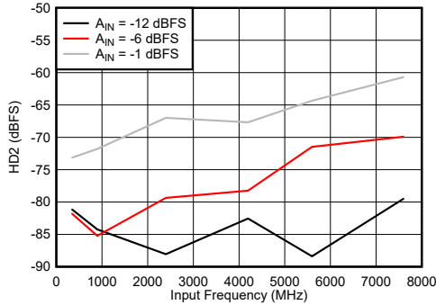
Figure 7-79. DES Mode: HD2 vs Input Frequency
