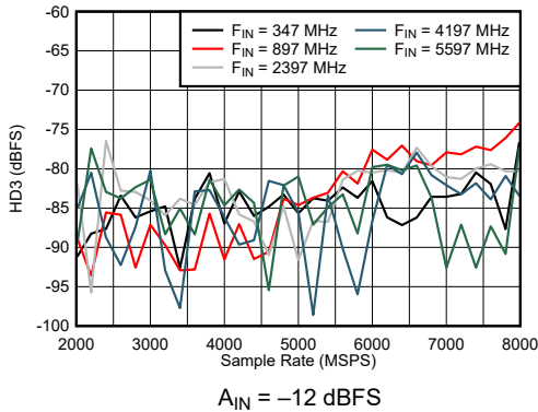
Figure 7-39. DES Mode: HD3 vs Sample Rate and Input Frequency
