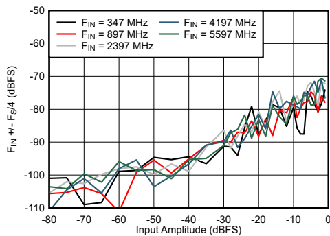
Figure 7-65. DES Mode: F_{\text{IN}} \pm F_{\text{IN}}/4 vs Input Amplitude and Frequency
