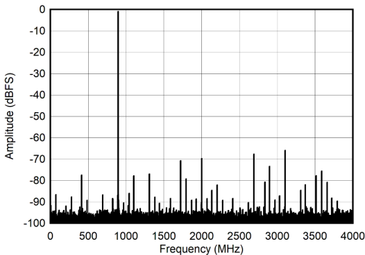
Figure 7-9. DES Mode: Single Tone FFT at 897 MHz
