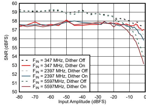
Figure 7-68. Dual Channel Mode: SNR vs Input Amplitude and Dither
