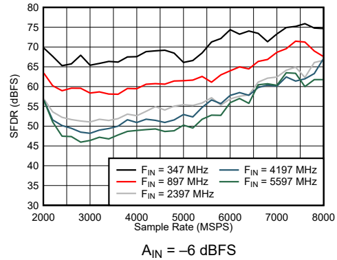
Figure 7-32. DES Mode: SFDR vs Sample Rate and Input Frequency
