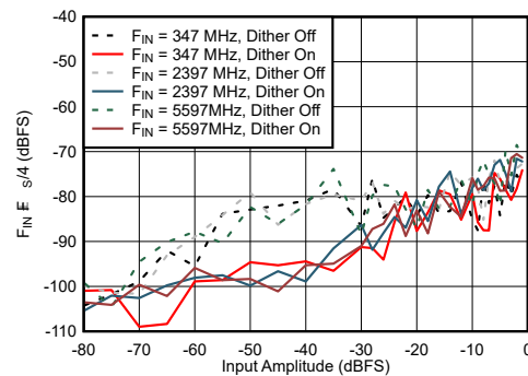
Figure 7-66. DES Mode: F_{\text{IN}} \pm F_{\text{IN}}/4 vs Input Amplitude and Dither
