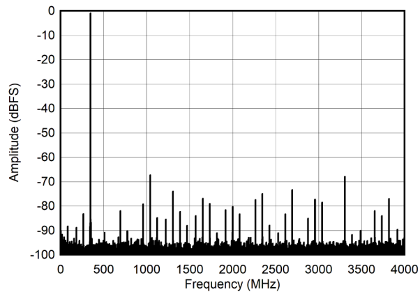
Figure 9-2. FFT for 347 MHz Input Signal, 8 GSPS, JMODE1
