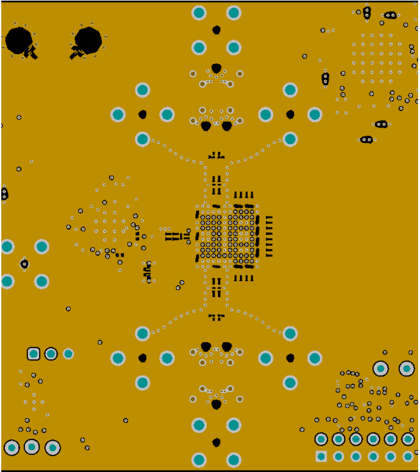
Figure 11-2. GND1 Cutouts to Optimize Impedance of Component Pads
