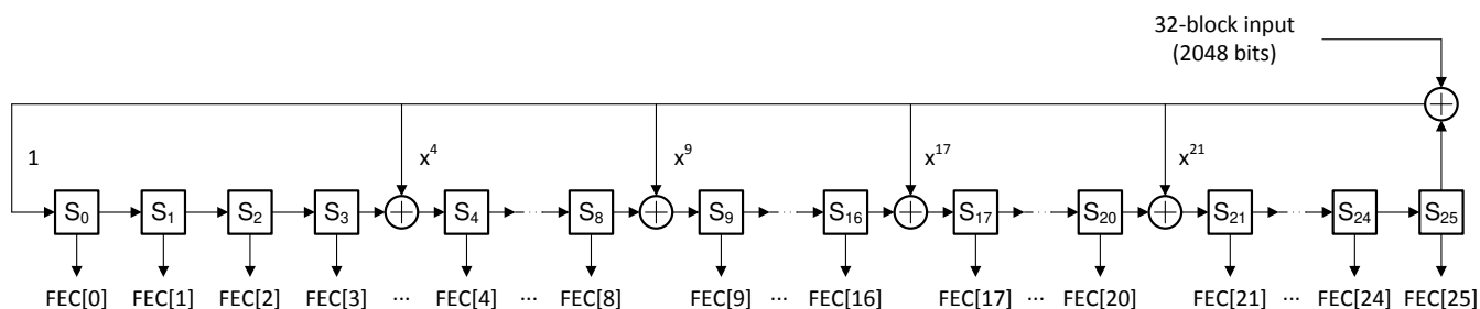
Figure 8-22. FEC Parity Bit Generator
