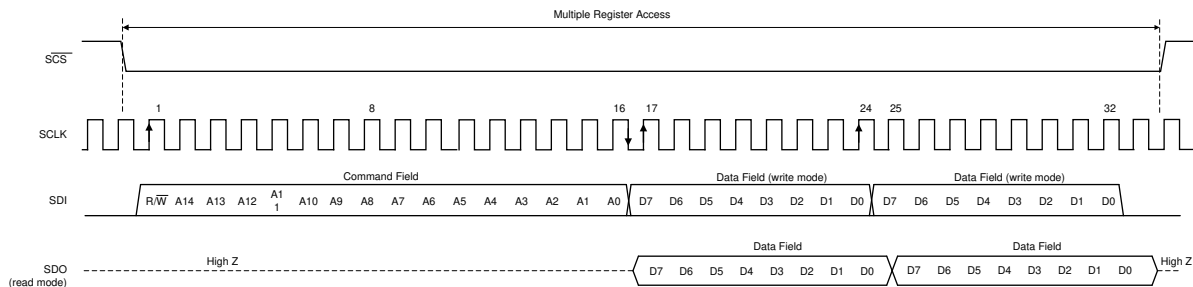
Figure 8-28. Serial Interface Protocol: Streaming Read/Write
