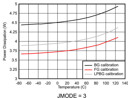
Figure 7-137. Dual Channel Mode: Power Dissipation vs Temperature
