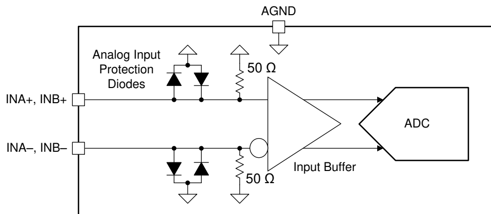
Figure 8-1. ADC12DJ4000RF Analog Input Internal Termination and Protection Diagram
