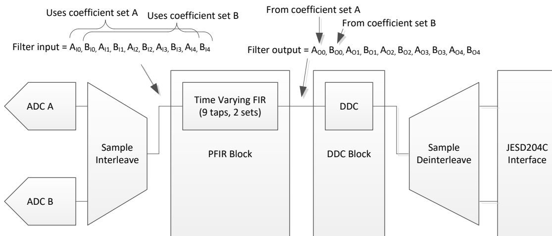
Figure 8-6. Time Varying Filter PFIR Block Diagram
