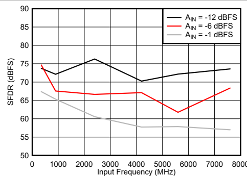
Figure 7-78. DES Mode: SFDR vs Input Frequency
