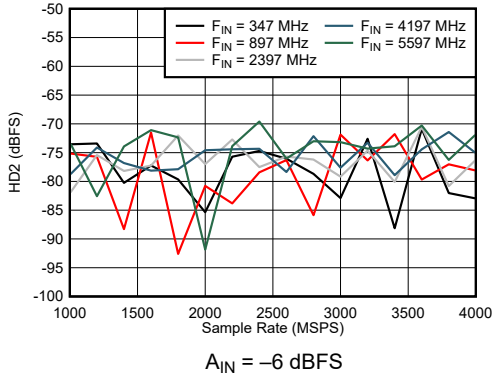
Figure 7-49. Dual Channel Mode: HD2 vs Sample Rate and Input Frequency
