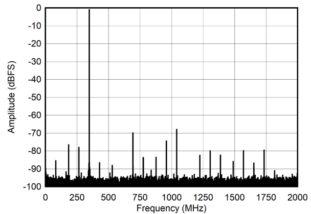
Figure 9-3. FFT for 347 MHz Input Signal, 4 GSPS, JMODE3
