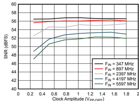
Figure 7-88. DES Mode: SNR vs Clock Amplitude
