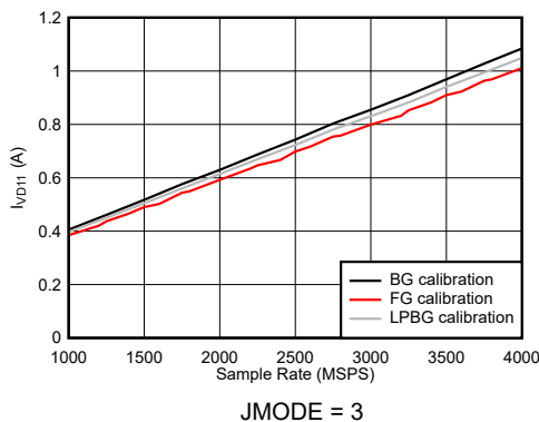
Figure 7-128. Dual Channel Mode: I_{VD11} vs Sample Rate
