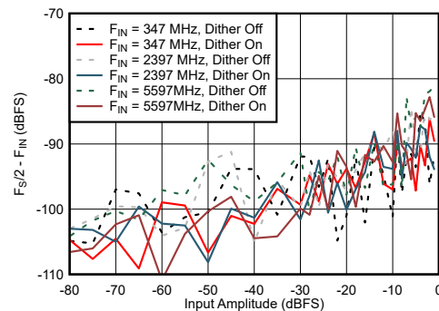
Figure 7-76. Dual Channel Mode: F_S/2 - F_{\text{IN}} vs Input Amplitude and Dither
