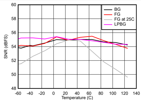
Figure 7-96. DES Mode: SNR vs Temperature and Calibration Mode FG25 is calibrated at 25°C and held at other temperatures, other modes recalibrated at each temperature
