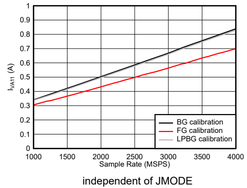
Figure 7-127. Dual Channel Mode: I_{VA11} vs Sample Rate
