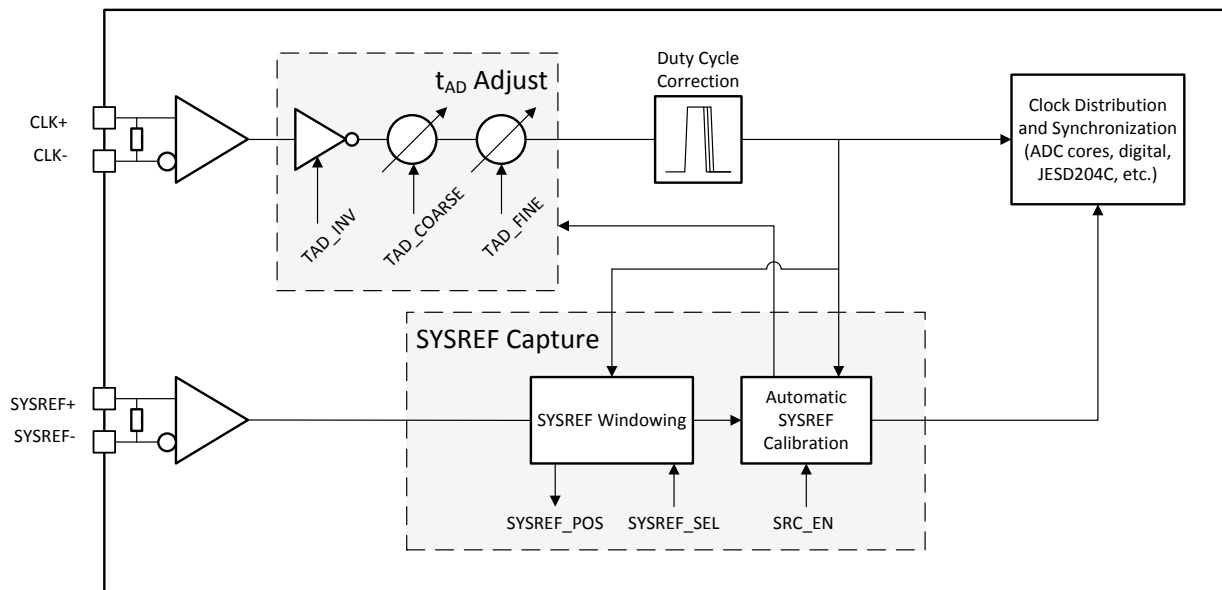
Figure 8-2. Clocking Subsystem
