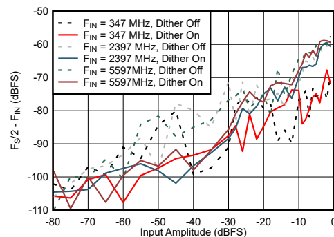
Figure 7-64. DES Mode: F_{\text{S}}/2 - F_{\text{IN}} vs Input Amplitude and Dither
