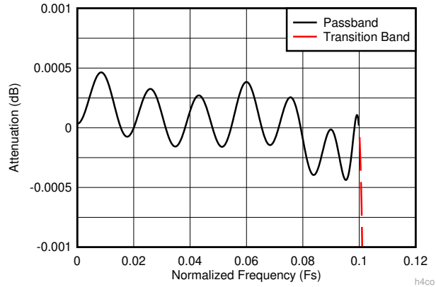
Figure 8-12. Decimate-by-4 Composite Zoomed Pass-Band Response
