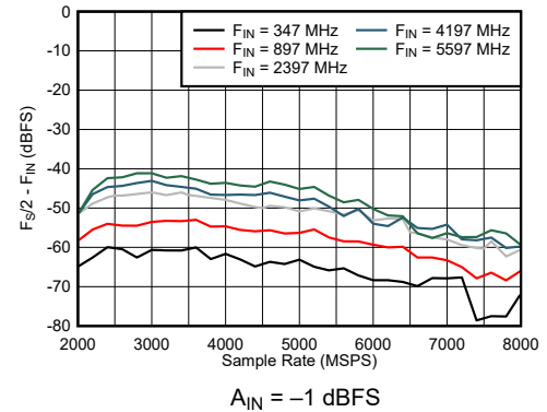
Figure 7-40. DES Mode: F_s/2 - F_{IN} vs Sample Rate and Input Frequency
