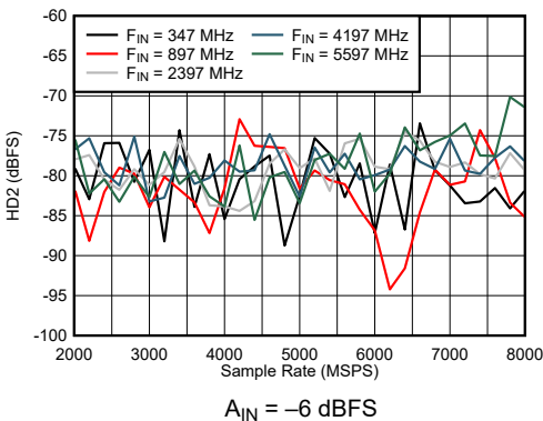
Figure 7-35. DES Mode: HD2 vs Sample Rate and Input Frequency
