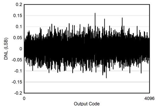
Figure 7-6. DNL vs ADC Code
