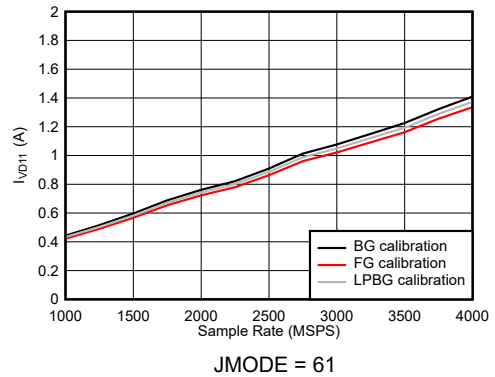
Figure 7-121. DES Mode: I_{VD11} vs Sample Rate
