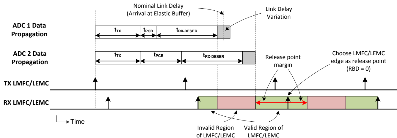
Figure 8-23. LMFC/LEMC Valid Region Definition for Elastic Buffer Release Point Selection
