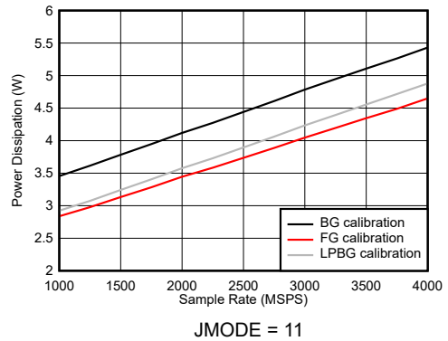
Figure 7-133. Dual Channel Mode: Power Dissipation vs Sample Rate
