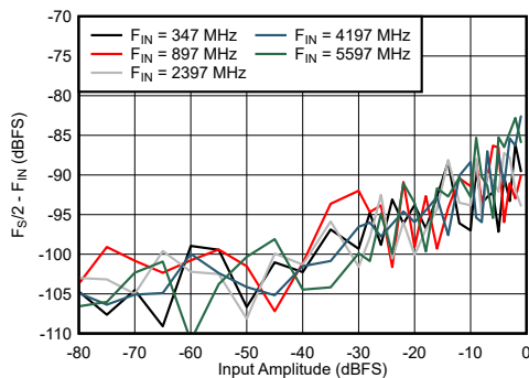
Figure 7-75. Dual Channel Mode: F_S/2 - F_{\text{IN}} vs Input Amplitude and Frequency
