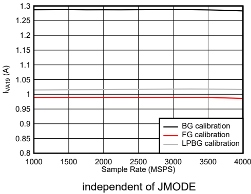
Figure 7-126. Dual Channel Mode: I_{VA19} vs Sample Rate
