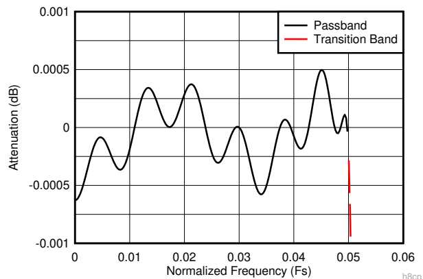
Figure 8-14. Decimate-by-8 Composite Zoomed Pass-Band Response
