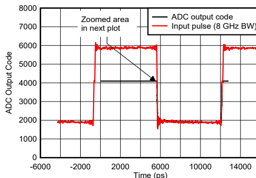
Figure 7-141. Pulse Overdrive Recovery
