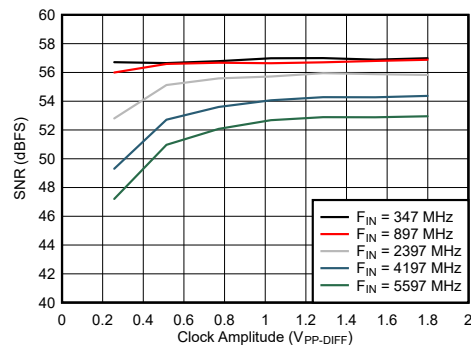
Figure 7-90. Dual Channel Mode: SNR vs Clock Amplitude
