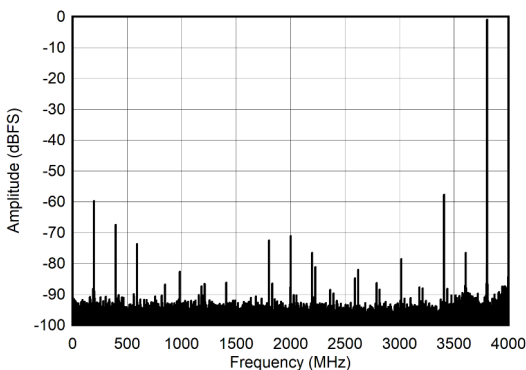
Figure 7-11. DES Mode: Single Tone FFT at 4197 MHz
