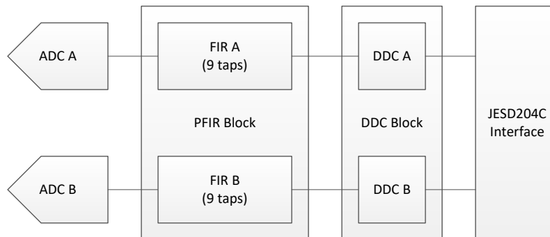
Figure 8-4. Dual Channel Equalization PFIR Block Diagram
