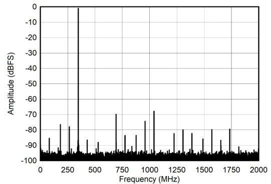
Figure 7-18. Dual Channel Mode: Single Tone FFT at 347 MHz
