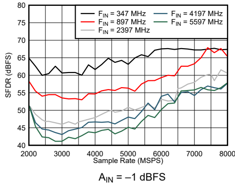
Figure 7-31. DES Mode: SFDR vs Sample Rate and Input Frequency
