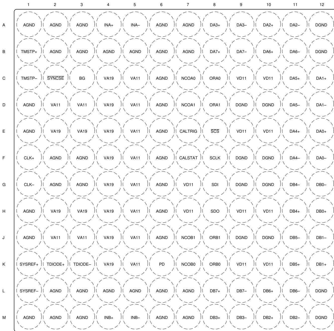
Figure 6-1. AAV Package, 144-Ball Flip Chip BGA, Top View
