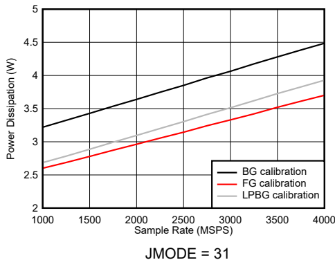
Figure 7-134. Dual Channel Mode: Power Dissipation vs Sample Rate
