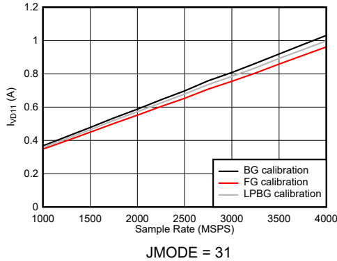
Figure 7-130. Dual Channel Mode: I_{VD11} vs Sample Rate
