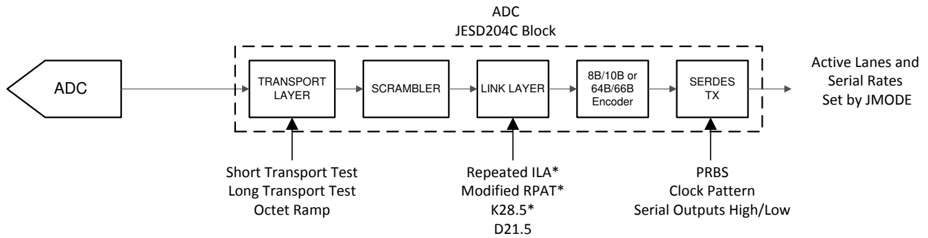
Figure 8-25. Test Mode Insertion Points
