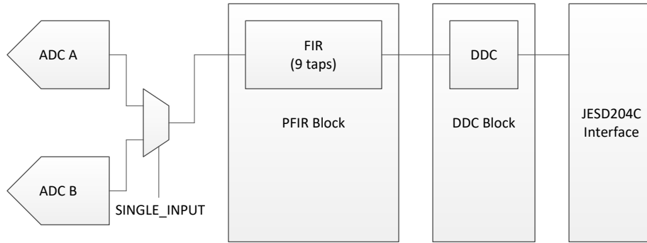
Figure 8-5. Single Channel Equalization PFIR Block Diagram
