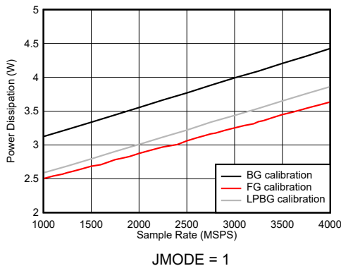
Figure 7-122. DES Mode: Power Dissipation vs Sample Rate
