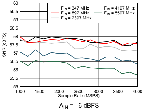
Figure 7-43. Dual Channel Mode: SNR vs Sample Rate and Input Frequency
