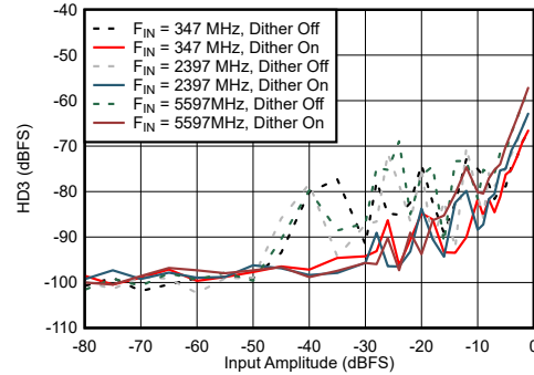
Figure 7-74. Dual Channel Mode: HD3 vs Input Amplitude and Dither
