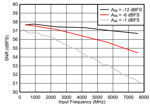
Figure 7-82. DES Mode: F_{\text{IN}} \pm F_S/4 vs Input Frequency
