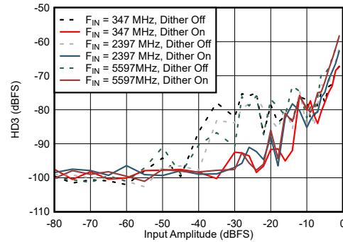
Figure 7-62. DES Mode: HD3 vs Input Amplitude and Dither
