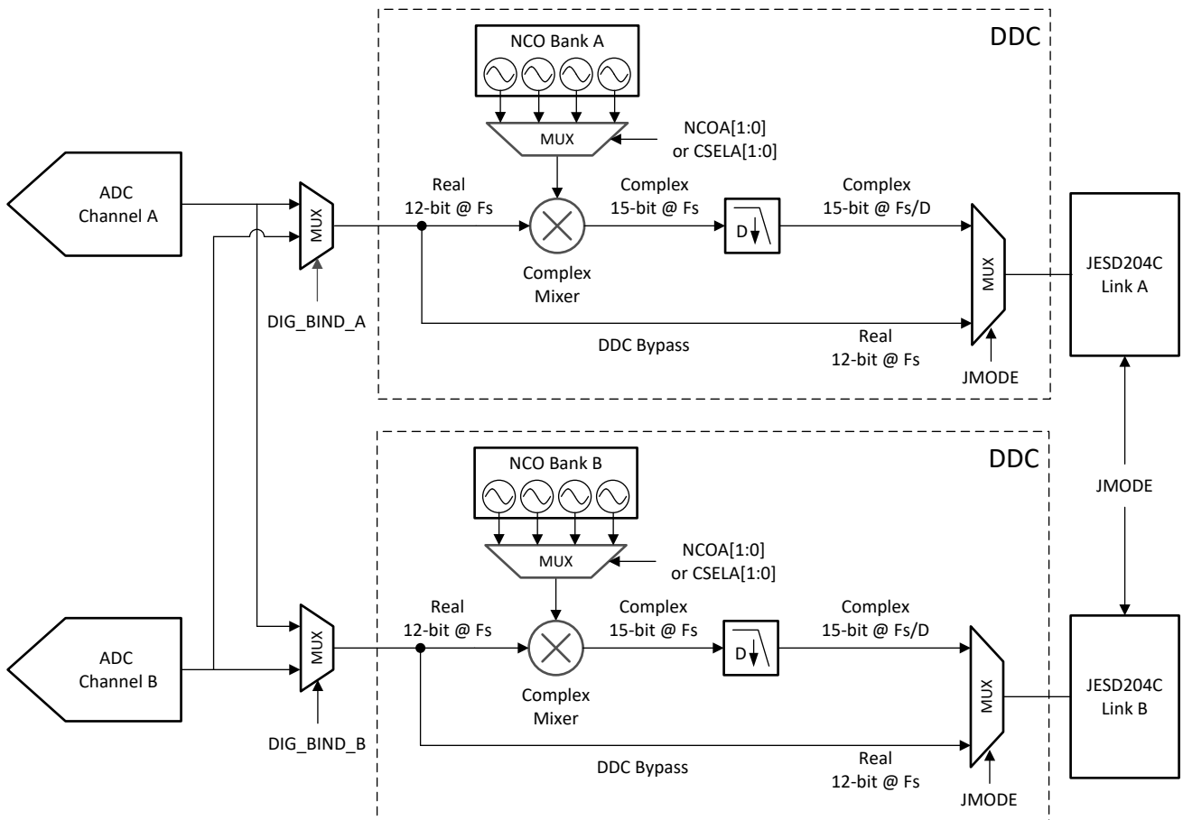
Figure 8-8. Digital Down Conversion Block in Dual Channel Mode
