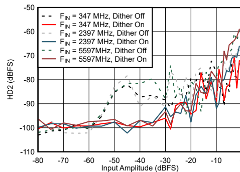
Figure 7-72. Dual Channel Mode: HD2 vs Input Amplitude and Dither
