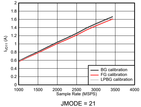
Figure 7-119. DES Mode: I_{VD11} vs Sample Rate
