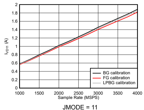
Figure 7-129. Dual Channel Mode: I_{VD11} vs Sample Rate
