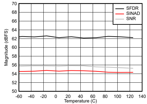
Figure 7-92. DES Mode: SNR, SINAD and SFDR vs Temperature FG calibration at each temperature
