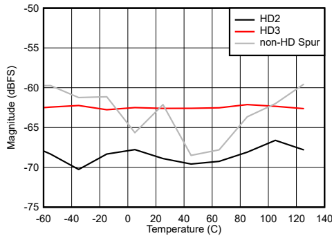
Figure 7-93. DES Mode: HD2, HD3 and Worst non-HD Spur vs Temperature FG calibration at each temperature
