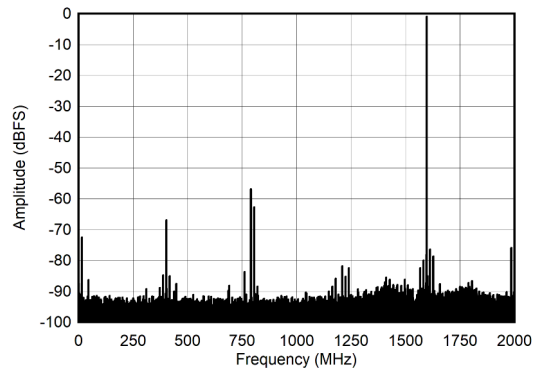
Figure 7-22. Dual Channel Mode: Single Tone FFT at 5597 MHz
