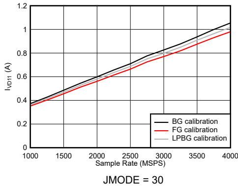
Figure 7-120. DES Mode: I_{VD11} vs Sample Rate
