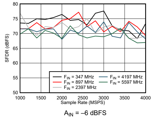
Figure 7-46. Dual Channel Mode: SFDR vs Sample Rate and Input Frequency
