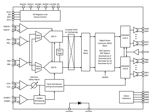
ADC12DJ4000RF Block Diagram
