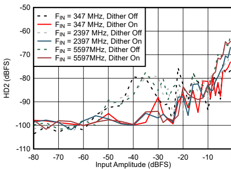
Figure 7-60. DES Mode: HD2 vs Input Amplitude and Dither
