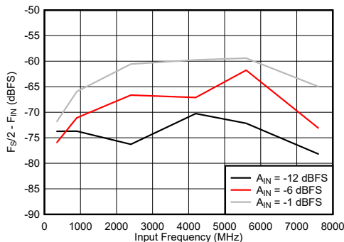
Figure 7-81. DES Mode: F_S/2 - F_{\text{IN}} vs Input Frequency
