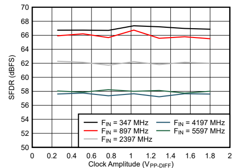
Figure 7-89. DES Mode: SFDR vs Clock Amplitude
