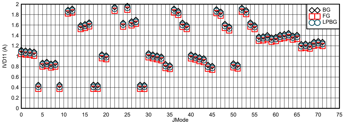
Figure 7-115. I_{V_{D11}} vs JMODE at F_{\text{CLK}} = 4\text{ GHz}
