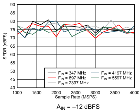
Figure 7-47. Dual Channel Mode: SFDR vs Sample Rate and Input Frequency
