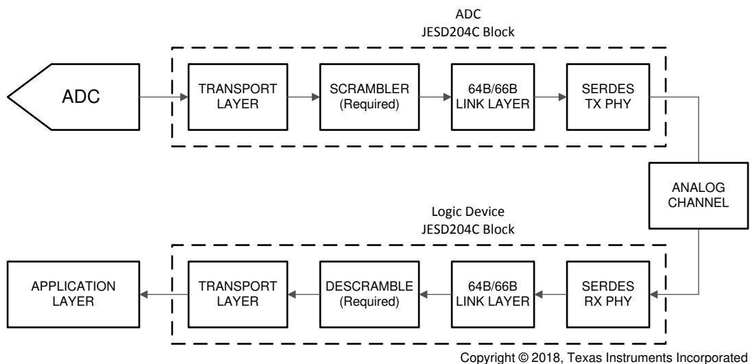
Figure 8-20. Simplified 64B/66B Encoded JESD204C Interface Diagram
