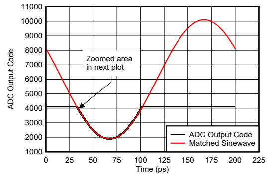
Figure 7-143. Sinewave Overdrive Recovery
