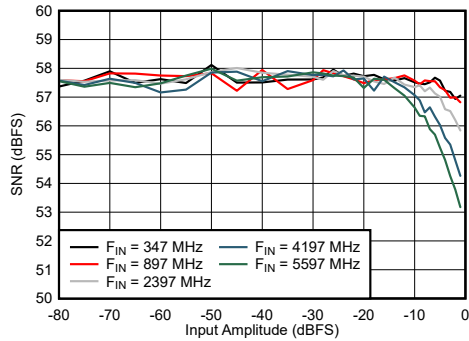
Figure 7-67. Dual Channel Mode: SNR vs Input Amplitude and Frequency
