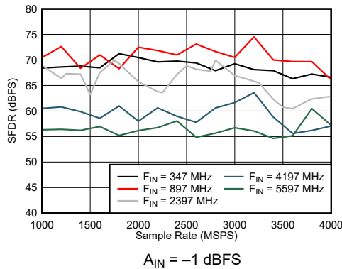
Figure 7-45. Dual Channel Mode: SFDR vs Sample Rate and Input Frequency
