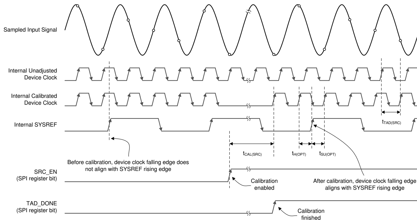
Figure 8-3. SYSREF Calibration Timing Diagram
