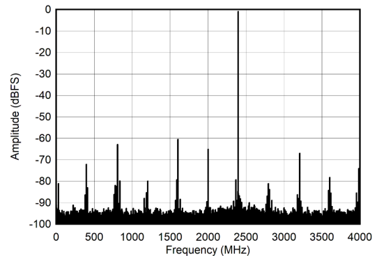
Figure 7-10. DES Mode: Single Tone FFT at 2397 MHz
