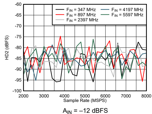
Figure 7-36. DES Mode: HD2 vs Sample Rate and Input Frequency
