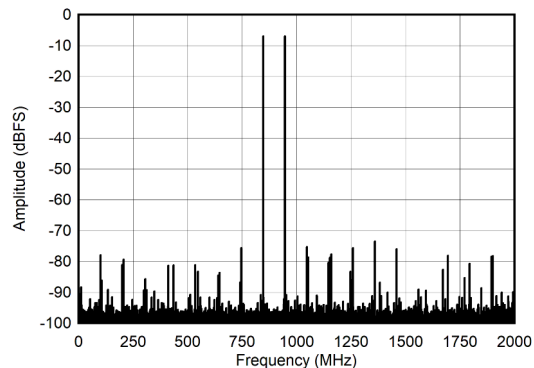
Figure 7-24. Dual Channel Mode: Two Tone FFT at 897 MHz
