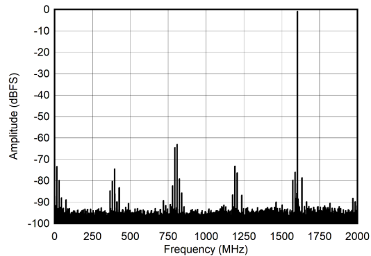
Figure 7-20. Dual Channel Mode: Single Tone FFT at 2397 MHz
