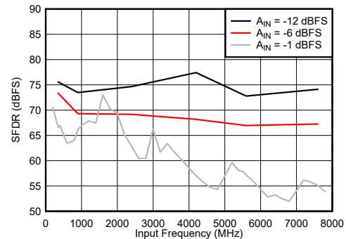
Figure 7-84. Dual Channel Mode: SFDR vs Input Frequency
