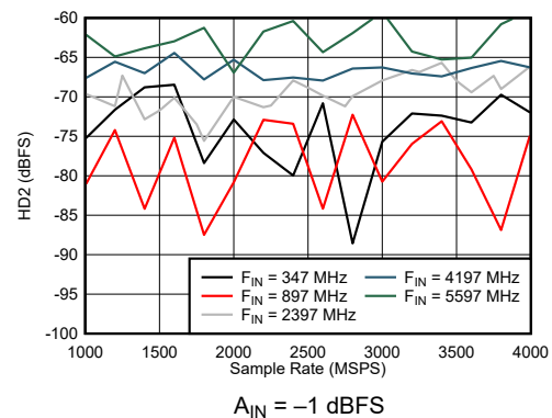
Figure 7-48. Dual Channel Mode: HD2 vs Sample Rate and Input Frequency
