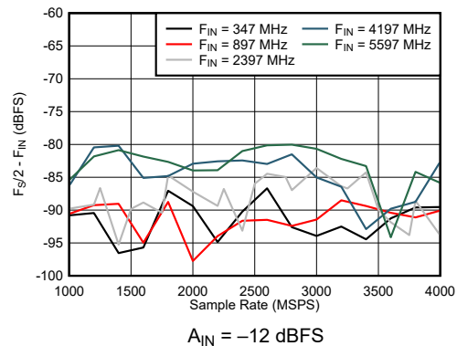
Figure 7-54. Dual Channel Mode: F_s/2 - F_{IN} vs Sample Rate and Input Frequency
