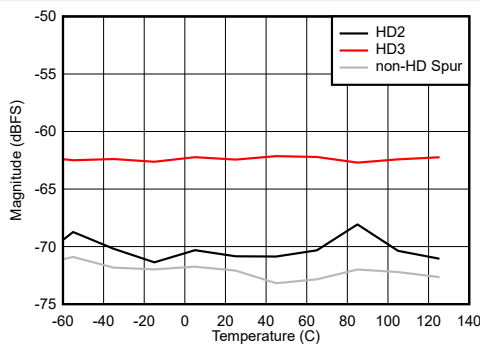
Figure 7-95. Dual Channel Mode: HD2, HD3 and Worst non-HD Spur vs Temperature FG calibration at each temperature
