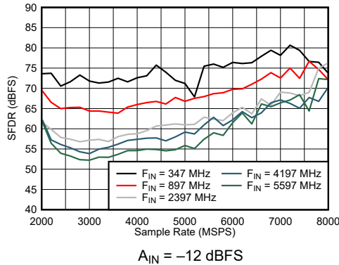
Figure 7-33. DES Mode: SFDR vs Sample Rate and Input Frequency
