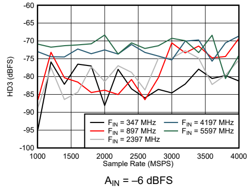
Figure 7-52. Dual Channel Mode: HD3 vs Sample Rate and Input Frequency
