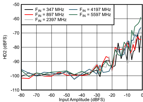
Figure 7-71. Dual Channel Mode: HD2 vs Input Amplitude and Frequency
