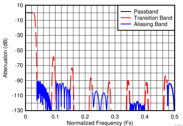
Figure 8-15. Decimate-by-16 Composite Response
