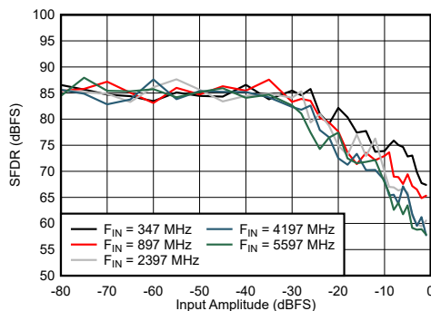
Figure 7-57. DES Mode: SFDR vs Input Amplitude and Frequency
