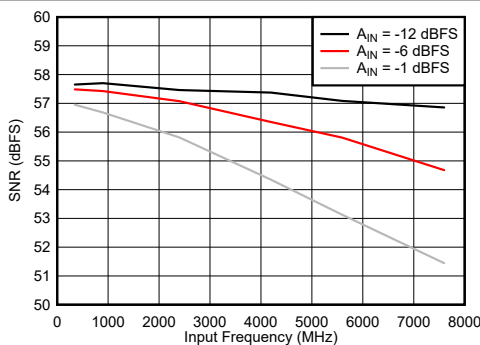
Figure 7-77. DES Mode: SNR vs Input Frequency
