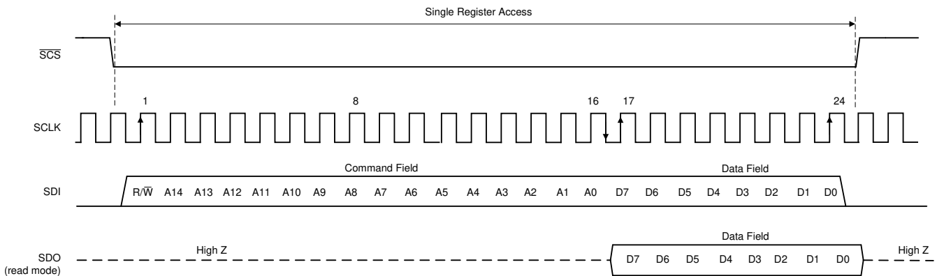
Figure 8-27. Serial Interface Protocol: Single Read/Write
