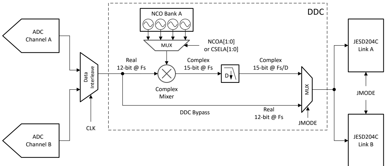
Figure 8-9. Digital Down Conversion Block in Single Channel Mode
