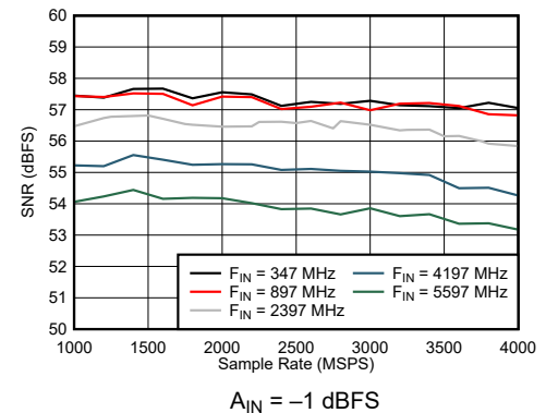
Figure 7-42. Dual Channel Mode: SNR vs Sample Rate and Input Frequency
