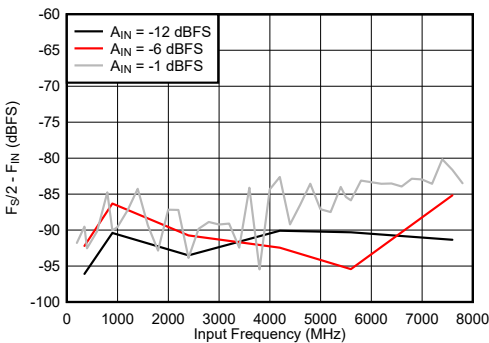
Figure 7-87. Dual Channel Mode: F_S/2 - F_{\text{IN}} vs Input Frequency
