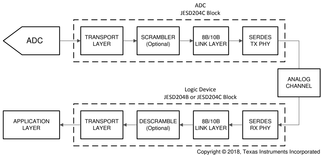
Figure 8-19. Simplified 8B/10B Encoded JESD204C Interface Diagram
