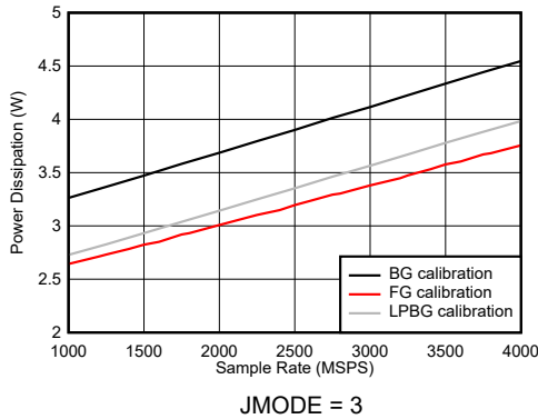
Figure 7-132. Dual Channel Mode: Power Dissipation vs Sample Rate
