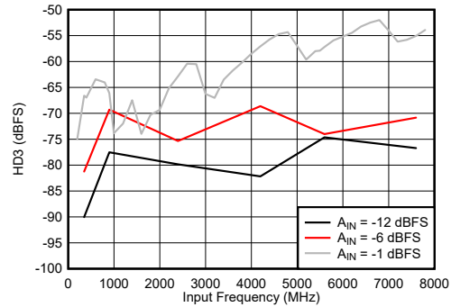
Figure 7-86. Dual Channel Mode: HD3 vs Input Frequency
