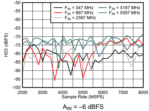
Figure 7-38. DES Mode: HD3 vs Sample Rate and Input Frequency
