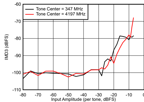
Figure 7-106. DES Mode: IMD3 vs Input Amplitude
