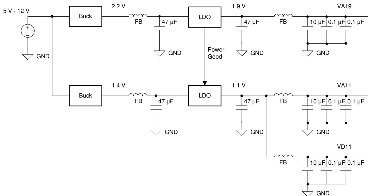
Figure 10-1. LDO Linear Regulator Approach Example
