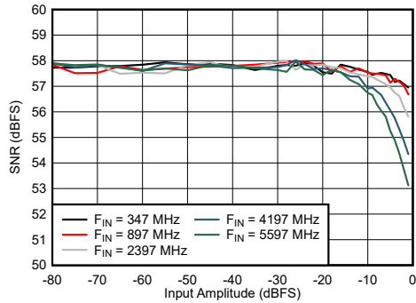
Figure 7-55. DES Mode: SNR vs Input Amplitude and Frequency
