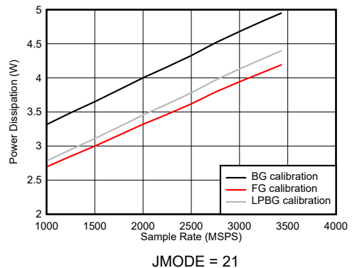
Figure 7-123. DES Mode: Power Dissipation vs Sample Rate
