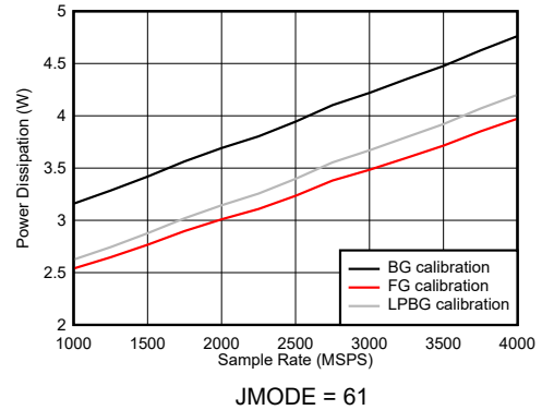
Figure 7-125. DES Mode: Power Dissipation vs Sample Rate
