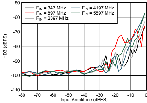
Figure 7-73. Dual Channel Mode: HD3 vs Input Amplitude and Frequency
