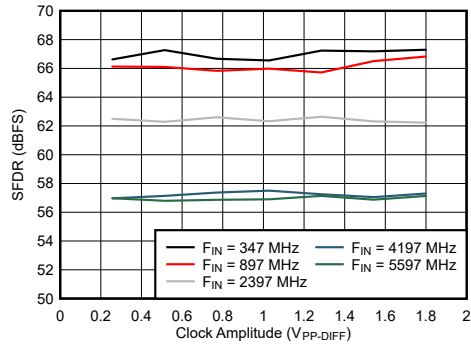
Figure 7-91. Dual Channel Mode: SFDR vs Clock Amplitude
