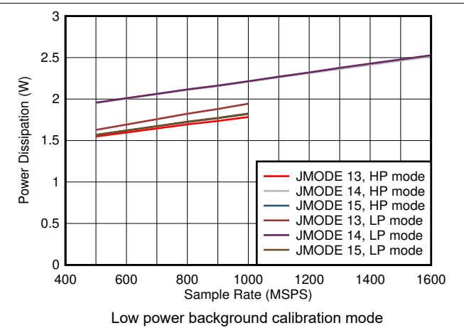
Figure 8-82. Quad Channel, Power Dissipation vs F_S and JMODE 13 - 15
