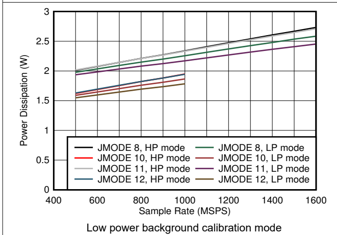
Figure 8-81. Quad Channel, Power Dissipation vs F_S and JMODE 8 - 12
