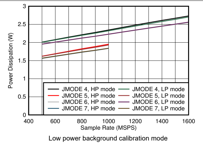
Figure 8-80. Quad Channel, Power Dissipation vs F_S and JMODE 4 - 7
