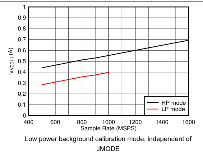
Figure 8-84. Quad Channel, I_{VA11} vs F_S
