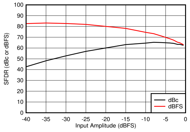
Figure 8-34. SFDR vs A_{IN}
