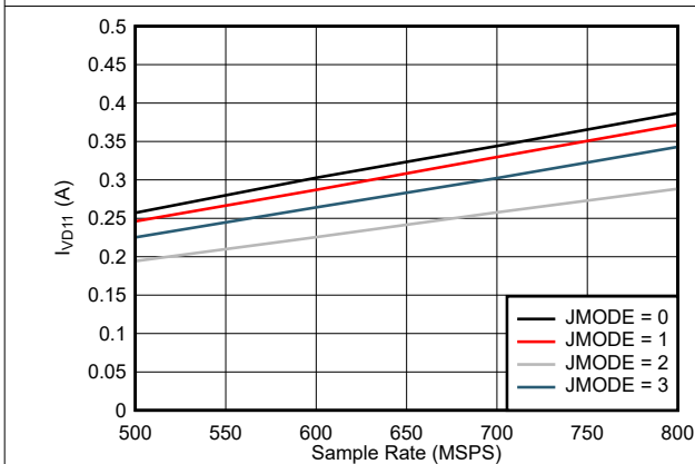
Figure 7-77. Quad Channel, I_{VD11} vs F_S for JMODES 0 - 3 Independent of Power Mode
