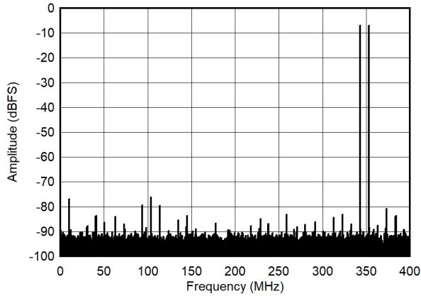
-7 dBFS each tone Figure 7-51. Single Tone FFT at 348 MHz
