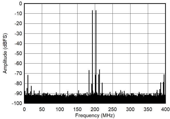
-7 dBFS each tone Figure 7-53. Single Tone FFT at 1798 MHz
