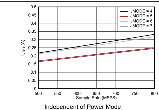
Figure 7-78. Quad Channel, I_{VD11} vs F_S for JMODES 4 - 7 Independent of Power Mode
