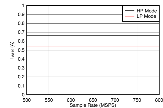
Figure 7-75. Quad Channel, I_{VA19} vs F_S Independent of JMODE
