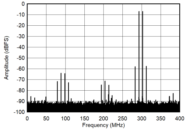
-7 dBFS each tone Figure 7-54. Single Tone FFT at 2698 MHz
