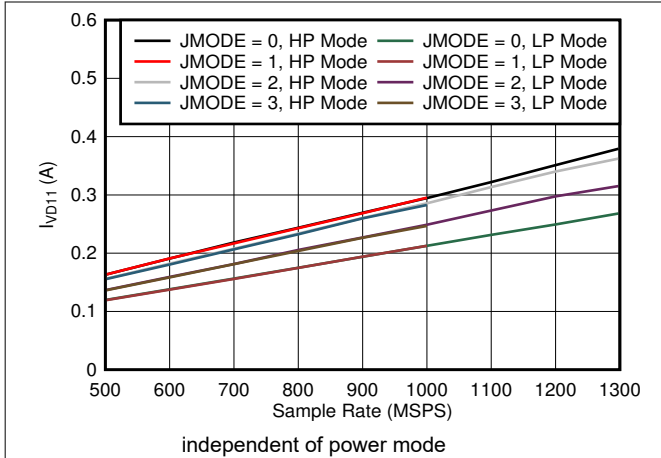
Figure 7-97. Dual Channel, I_{VD11} vs FS and JMODE 0 - 3
