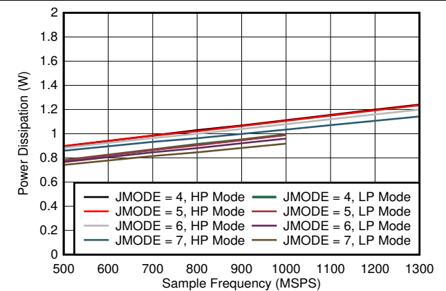
Figure 7-102. Single Channel, Power Dissipation vs FS for JMODES 4 - 7
