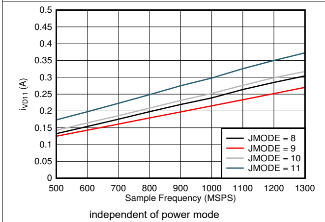
Figure 7-99. Dual Channel, I_{VD11} vs FS and JMODE 8 - 11
