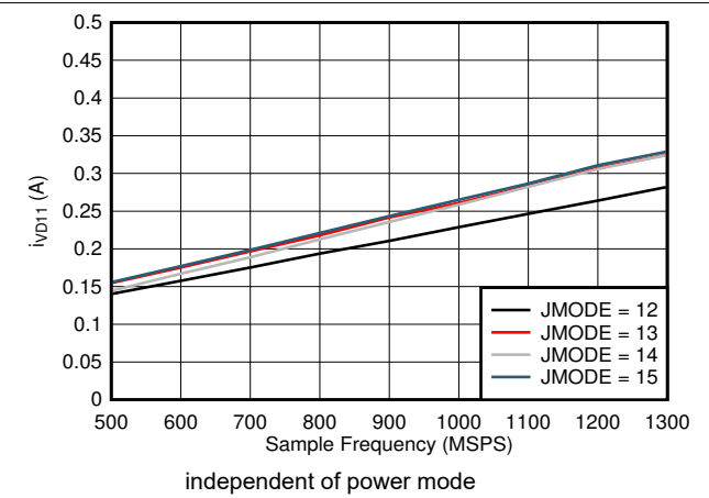
Figure 7-100. Dual Channel, I_{VD11} vs FS and JMODE 12 - 15
