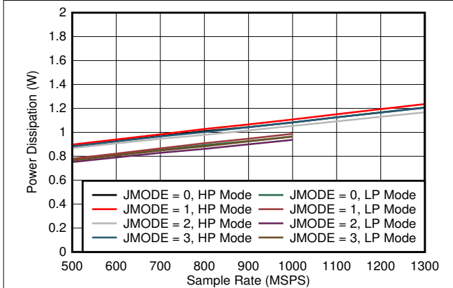
Figure 7-101. Single Channel, Power Dissipation vs FS for JMODES 0 - 3
