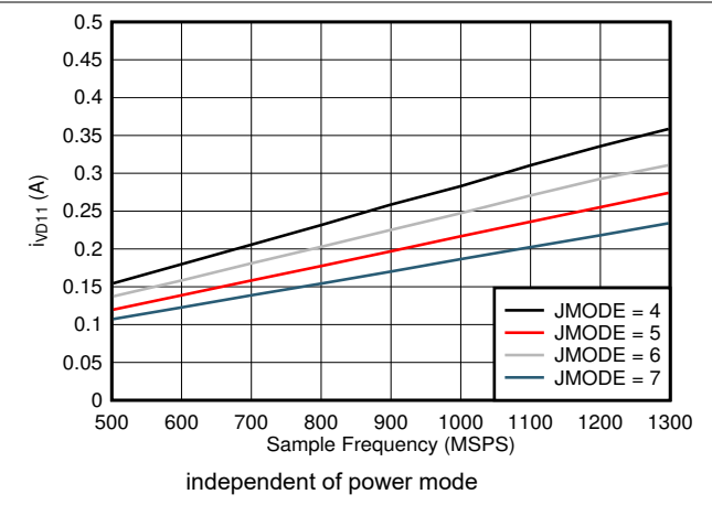
Figure 7-98. Dual Channel, I_{VD11} vs FS and JMODE 4 - 7
