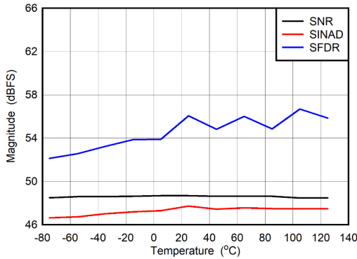
Figure 6-85. DES Mode: SNR, SINAD and SFDR vs Temperature
