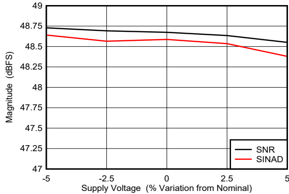
Figure 6-95. Dual Channel Mode: SNR and SINAD vs Supply Voltage
