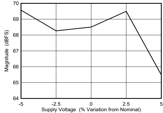
Figure 6-96. Dual Channel Mode: SFDR vs Supply Voltage
