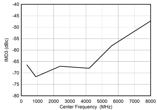
Figure 6-100. DES Mode: IMD3 vs Input Frequency
