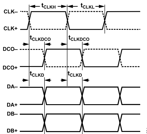
Figure 4. Data Output Timing Diagram
