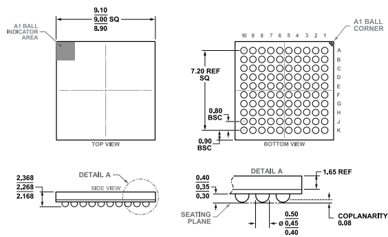
Figure 90. 100-Ball Chip Scale Package Ball Grid Array [CSP_BGA] (BC-100-7) Dimensions shown in millimeters
