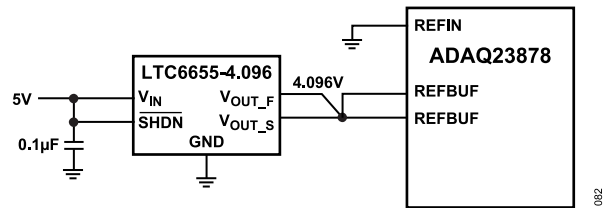
Figure 83. Overdriving REFBUF Using the LTC6655
